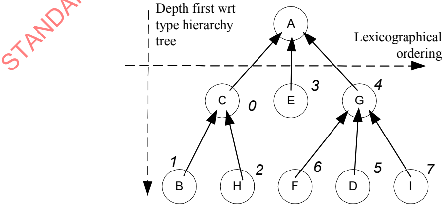
Figure 9 — Example for the Type Identification Code assignment for the types derived from A
