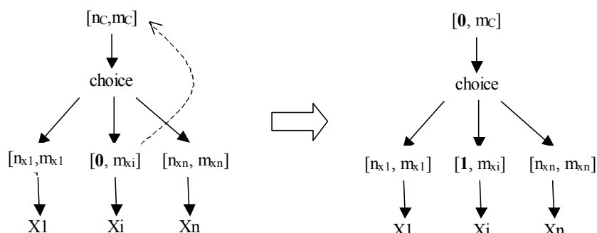
Figure 19 — Empty choice simplification rule
