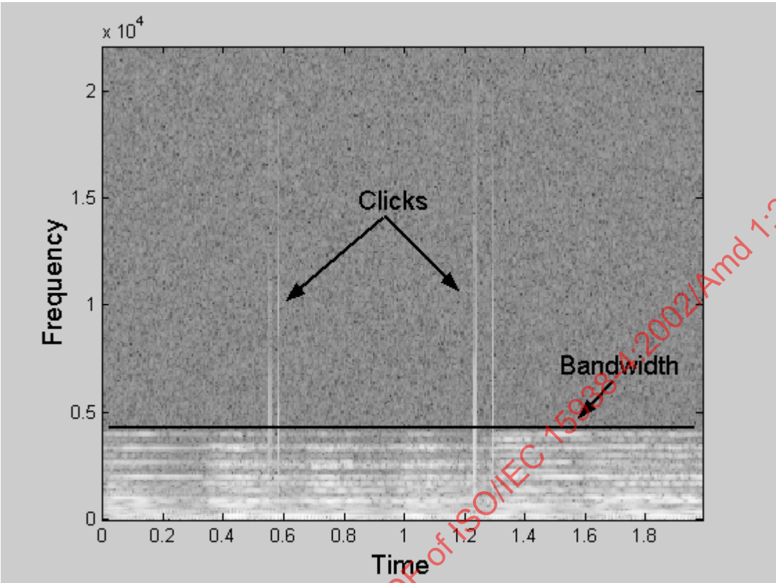
Figure AMD1-3 - Spectrogram of a degraded audio file
