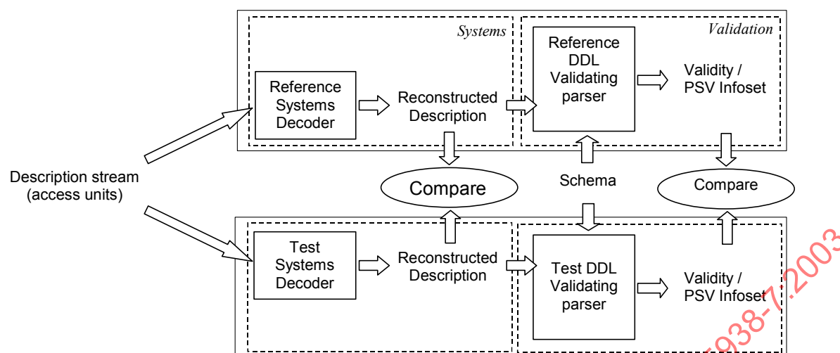
Figure 4 — Overview of conformance testing of systems based validating terminals
