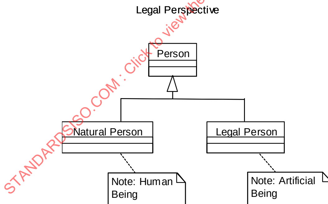
Figure E.18 — UML-based representation of "Figure E.17: Generic legal perspective of "Person""
