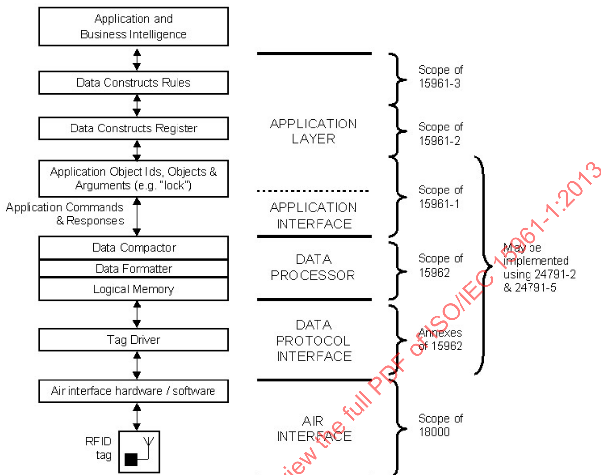
Figure 1 — Schematic of protocol layers for an implementation of RFID for item management
