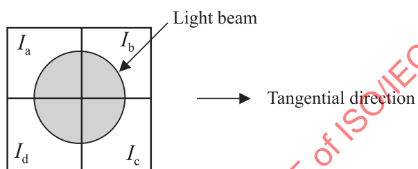
Figure 12 - Cross-track signal
