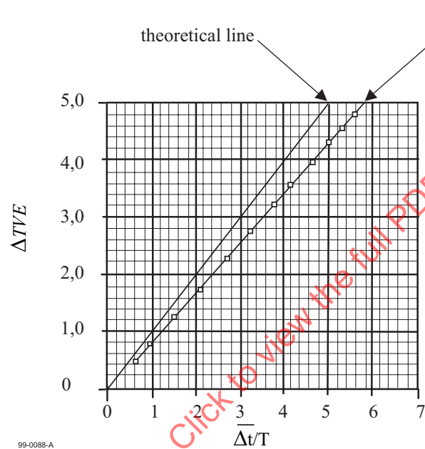
Figure C.3 - \Delta t/T vs \Delta TVE
