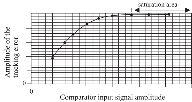
Figure C.2 - Comparator input signal amplitude vs tracking error signal amplitude
