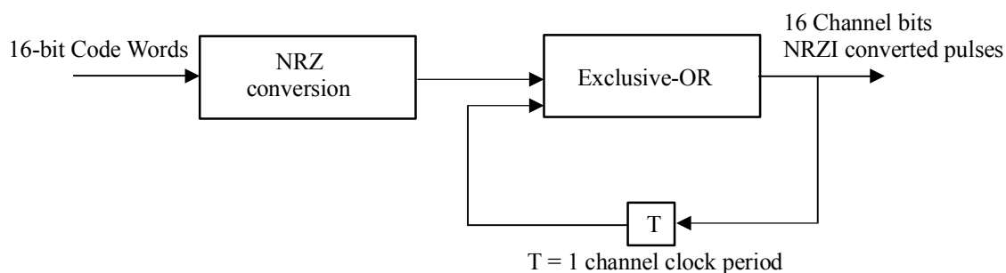
Figure 22 - NRZI conversion
