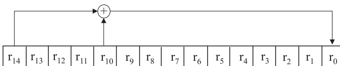
Figure 19 - Feedback shift register
