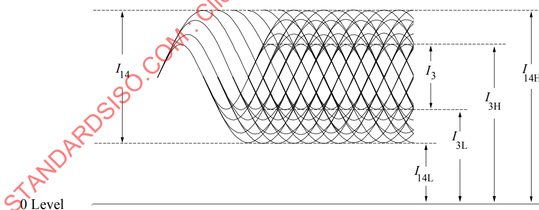
Figure 11 - Modulated amplitude
