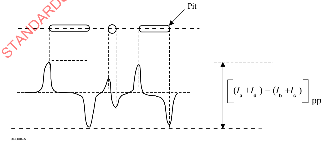
Figure 15 - Tangential push-pull signal
