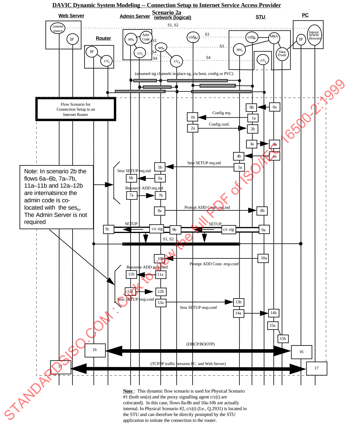
Figure 9.5-16 - DAVIC Dynamic System Model - Establishment of Direct Access to Internet for Direct Internet Scenario 2a
