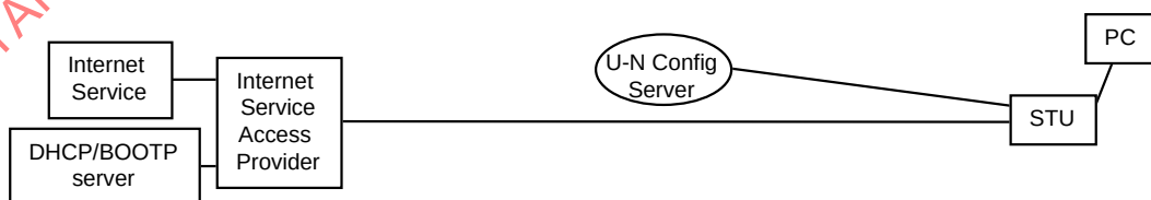
Figure 9.5-7 – System level Connectivity for Direct Internet Scenario 1a
