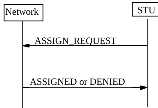
Figure 8.5 — DIIP message sequence
