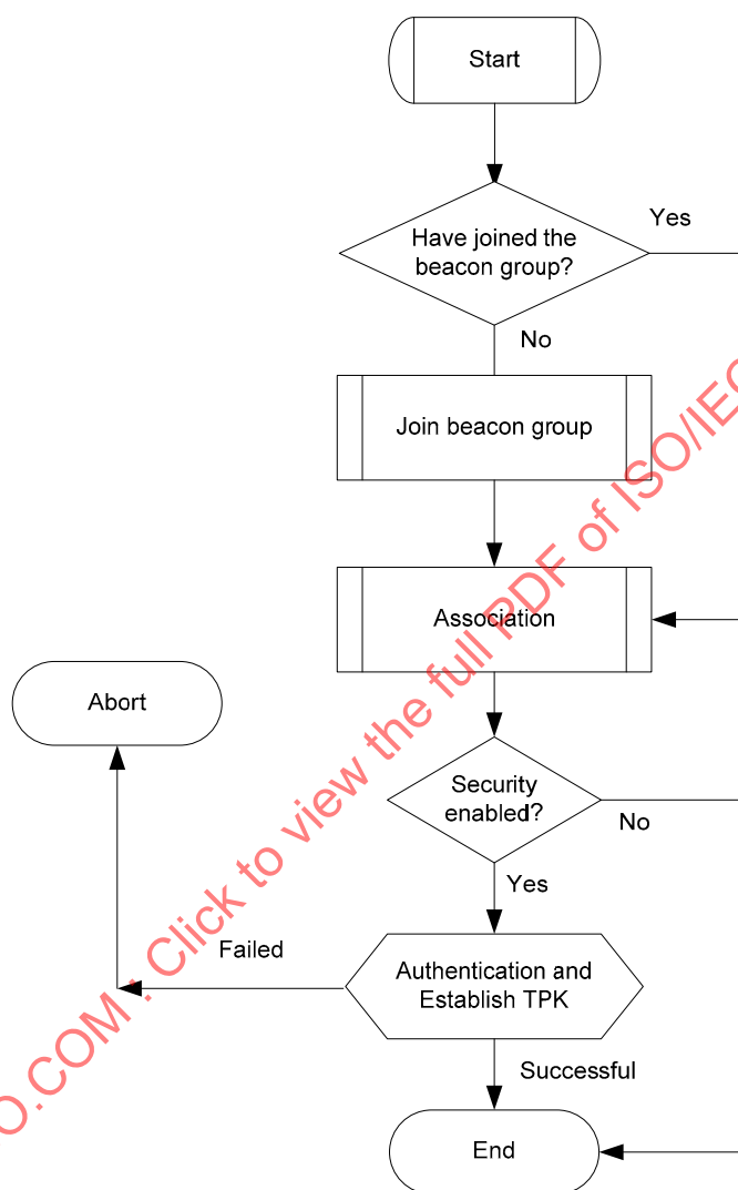
Figure 25 — Pairing Procedure
