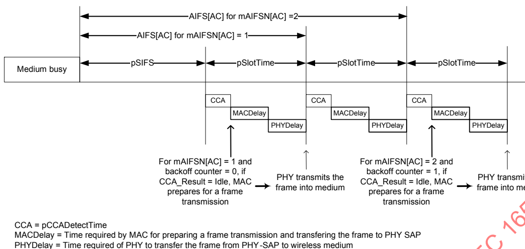
Figure 16 — PCA timing relationships
