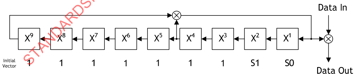
Figure 36 — Data scrambler
