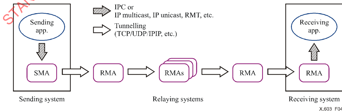
Figure 4 – RMCP data transport model
