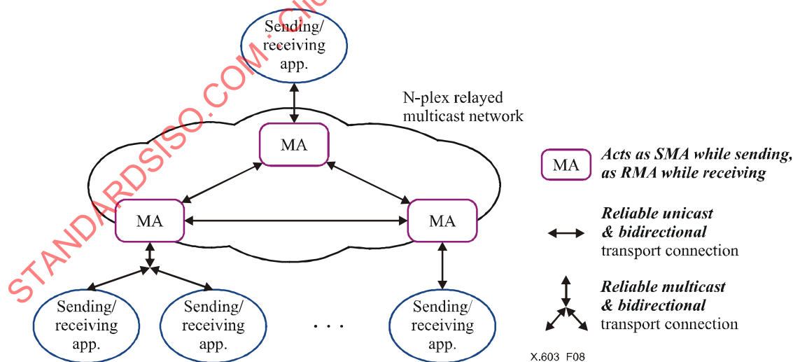
Figure 8 – N-plex reliable data delivery model
