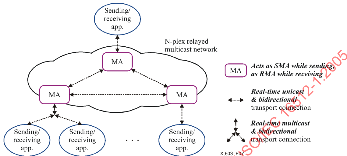
Figure 7 – N-plex real-time data delivery model
