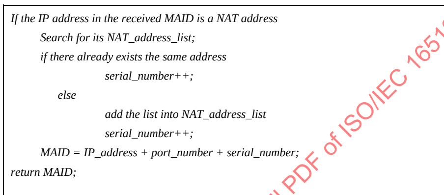
Figure 34 – A simple algorithm to generate a unique MAID
