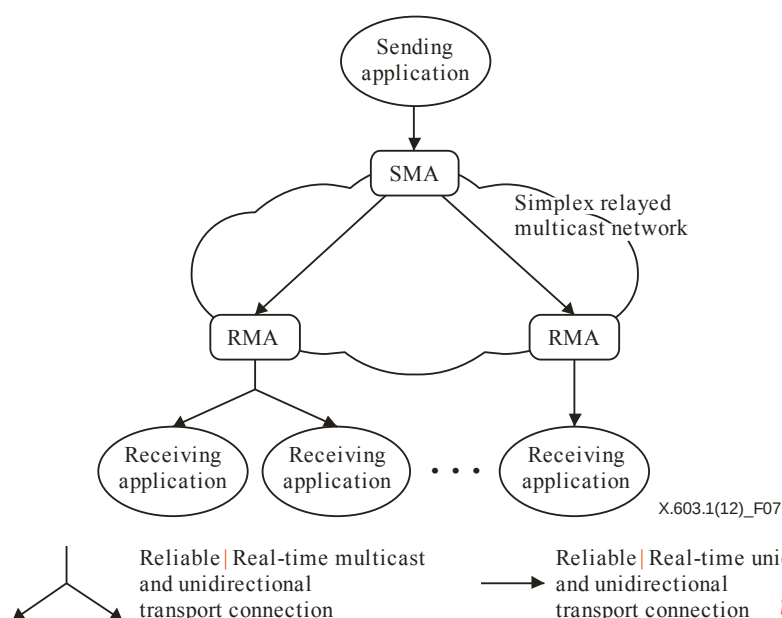
Figure 7 – Relayed multicast tree configured by RMCP-2
