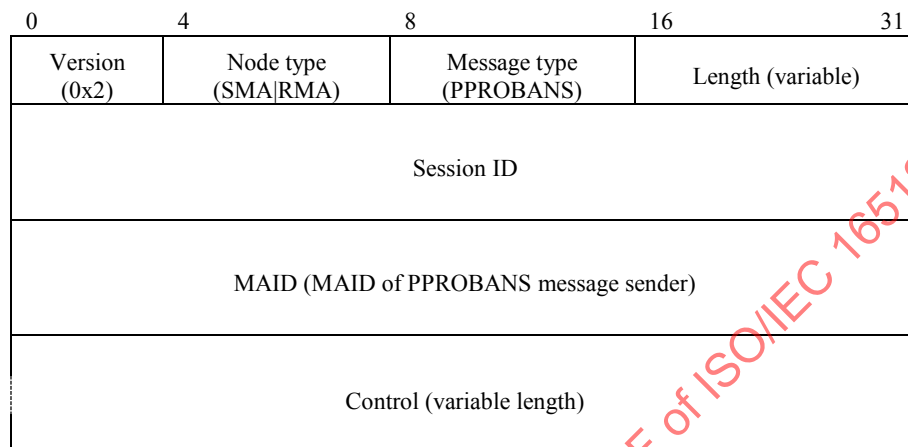
Figure 61 – PPROBANS message format
