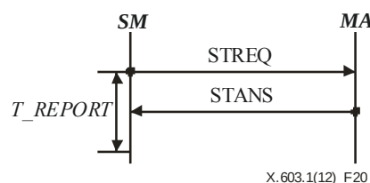
Figure 20 – MA monitoring – Status report
