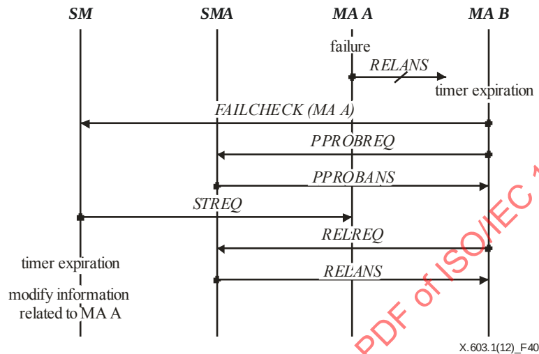
Figure 40 – PMA failure detection and recovery
