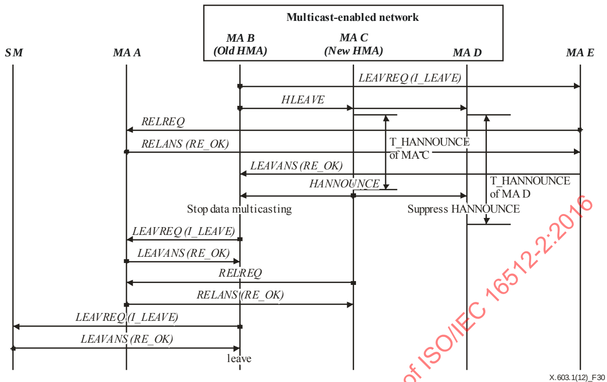
Figure 30 – HMA leave in a multicast network
