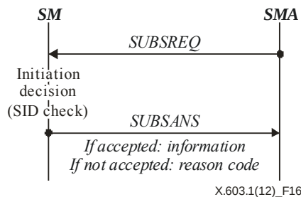
Figure 16 – RMCP-2 session initiation
