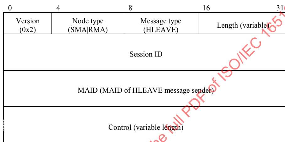
Figure 64 – HLEAVE message format
