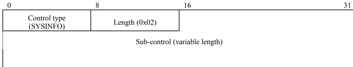
Figure 93 – SYSINFO control format
