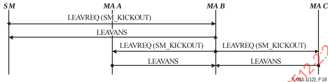
Figure 18 – SM's expulsion of MA B
