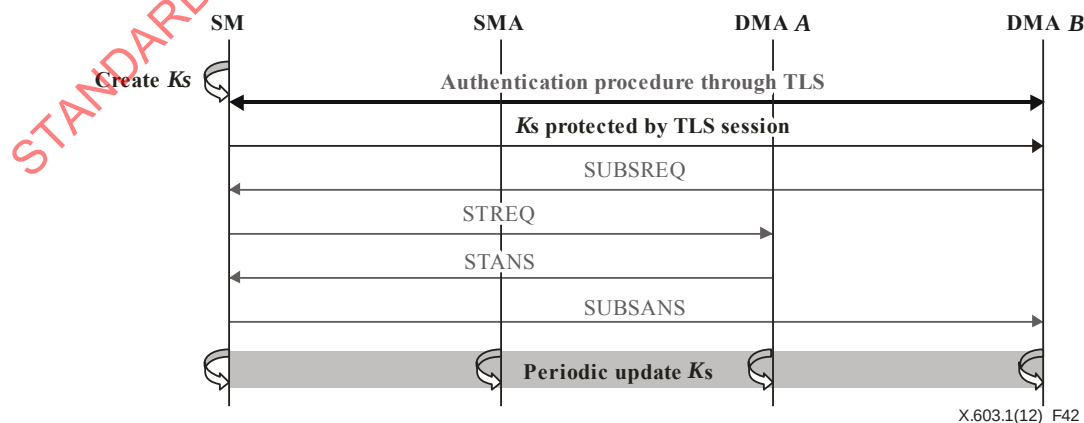
Figure 42 – Session key management
