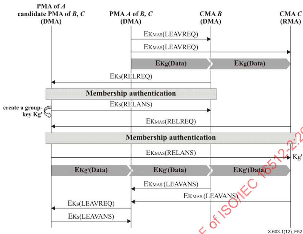
Figure 52 – DMA leave in a unicast network
