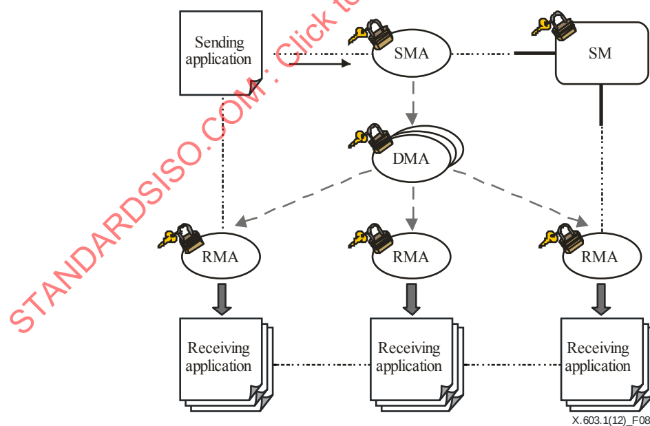
Figure 8 – RMCP-2 service topology with security
