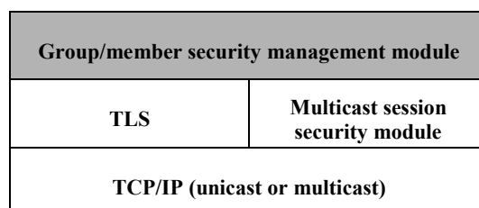
Figure 13 – The group/member security management module of an MA of a secure RMCP-2
