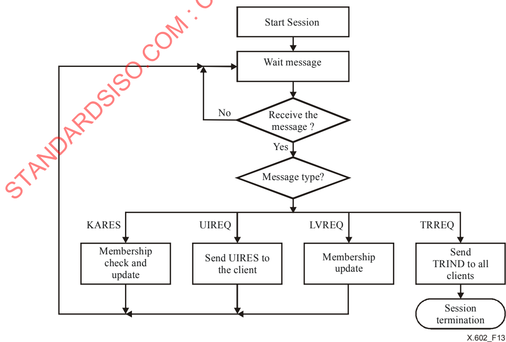
Figure 13 – GMP server (MM) operation algorithm
