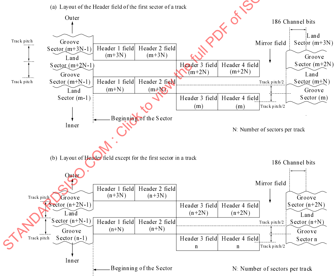
Figure 18 - Layout of Header field in the Rewritable Area
