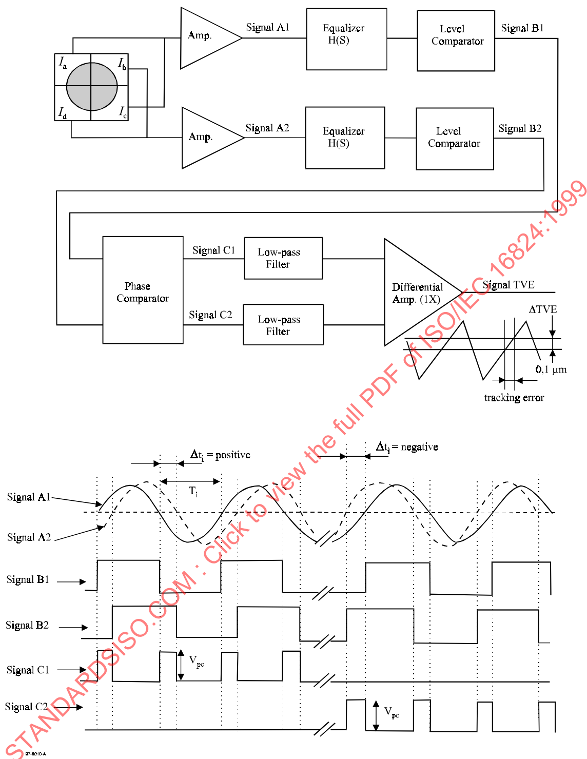
Figure C.1 - Circuit for tracking error measurements
