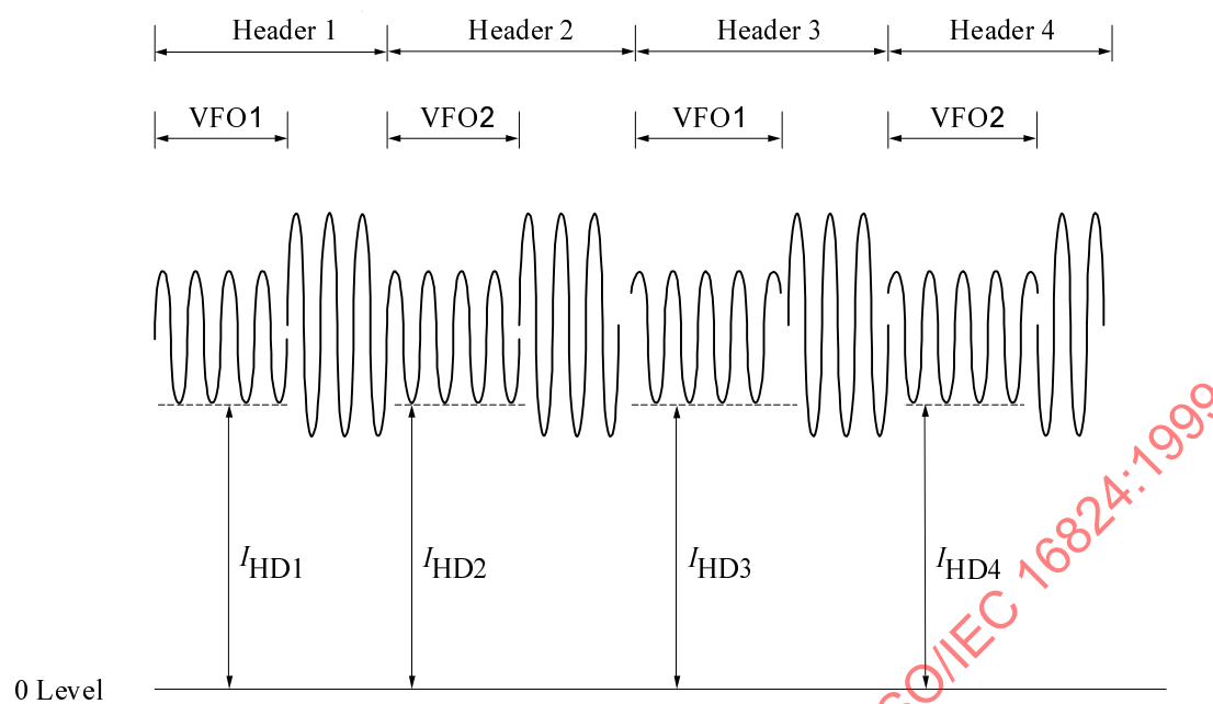
Figure 41 - Signals from Header 1, Header 2, Header 3 and Header 4 in Read channel 1
