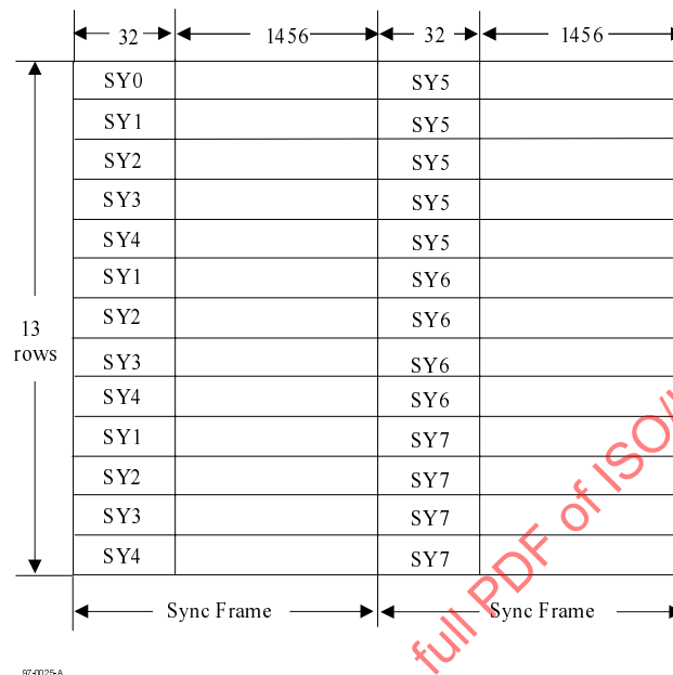
Figure 16 - Recorded Data Field
