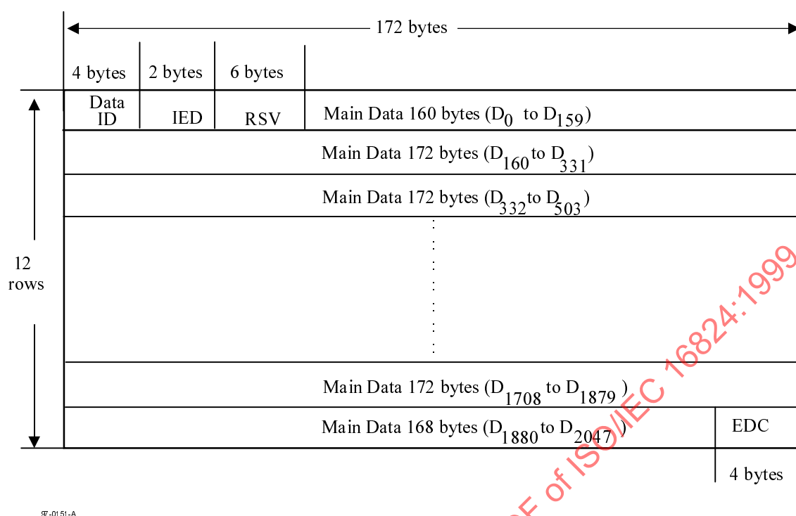
Figure 9 - Data Frame
