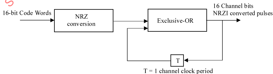
Figure 15 - NRZI conversion
