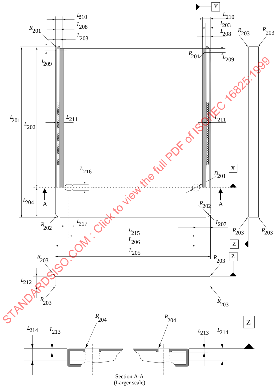
Figure 13 - Overall dimensions
