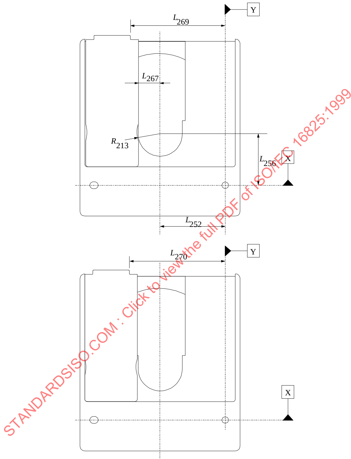
Figure 20 - Shutter in just left-hand open position (top) and maximum left-hand open position (bottom)
