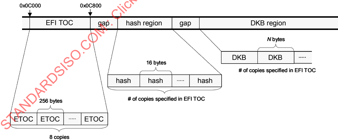
Figure B.1 — Example lay-out of Extended format information in ADIP
