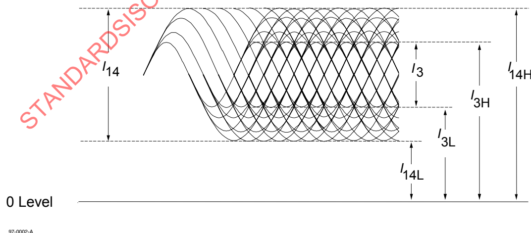
Figure 27 — Signals from spaces and marks in Read channel 1
