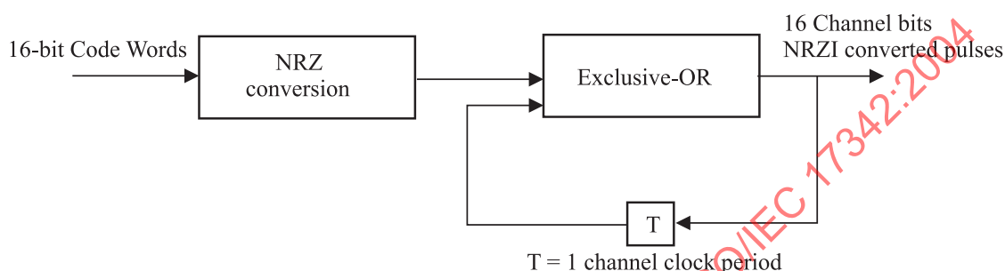
Figure 29 - NRZI conversion
