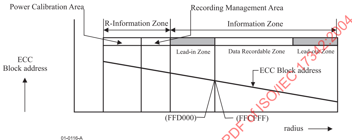
Figure 43 - Pre-pit sector layout and ECC Block numbering
