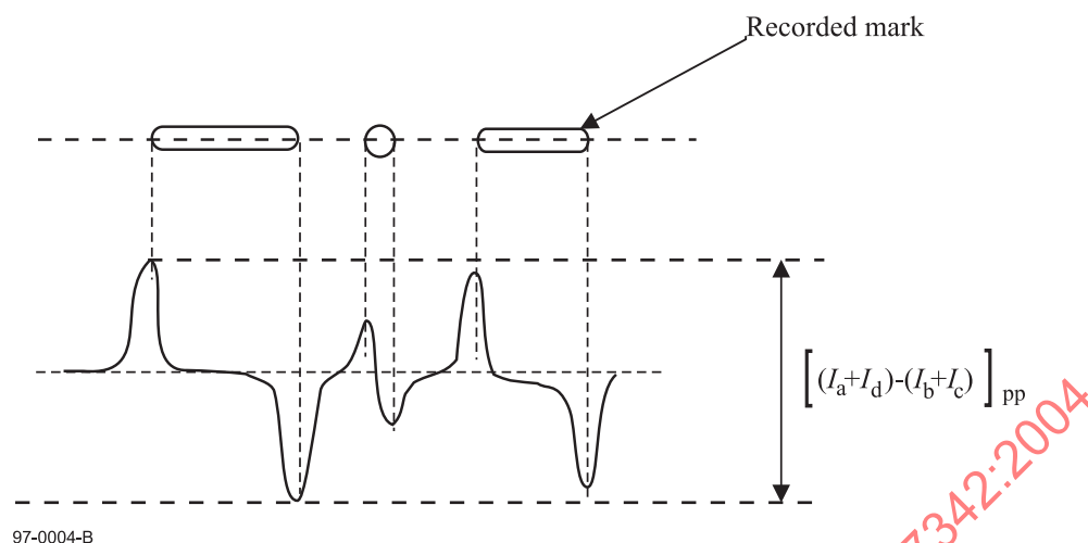
Figure 14 - Tangential push-pull signal
