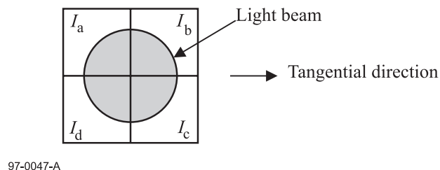
Figure 17 - Quadrant photo detector
