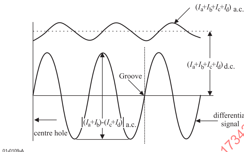
Figure 22 - Radial push-pull tracking error signal
