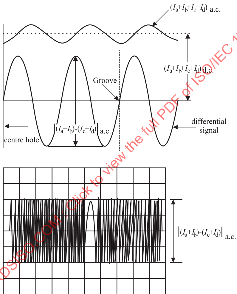
Figure 18 - Radial push-pull tracking error signal
