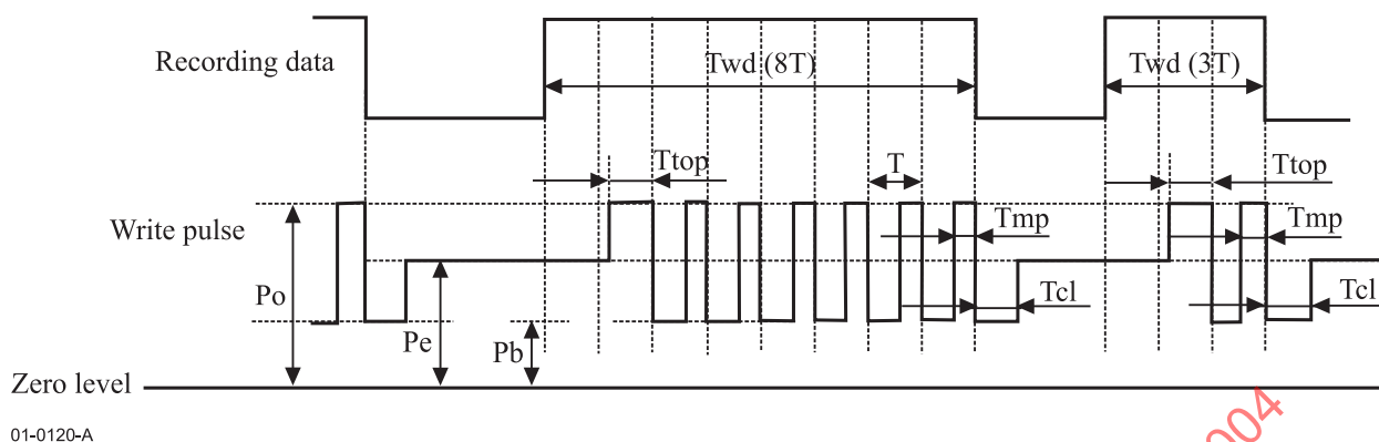
Figure 16 - Basic write strategy
