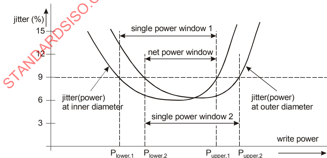
Figure 31 - Example of the write power windows
