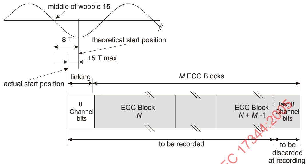
Figure 17 - Recording Unit
