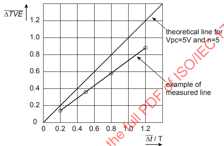
Figure E.3 - \overline{\Delta TVE} versus \overline{\Delta t}/T
