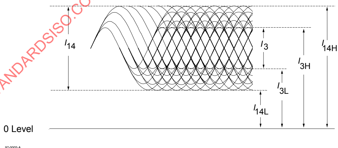
Figure 32 — Signals from spaces and marks in Read channel 1
