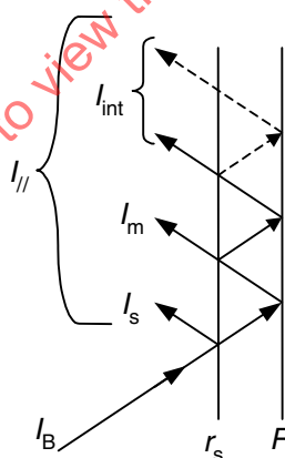
Figure C.1 — Reflectivity calibration
