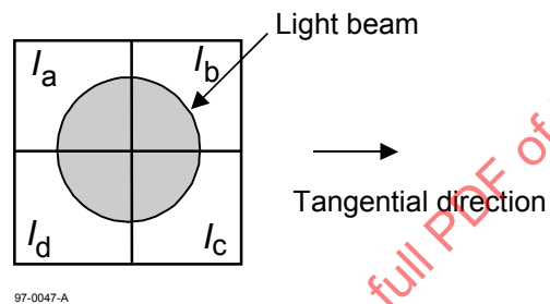
Figure 33 — Quadrant photo detector
