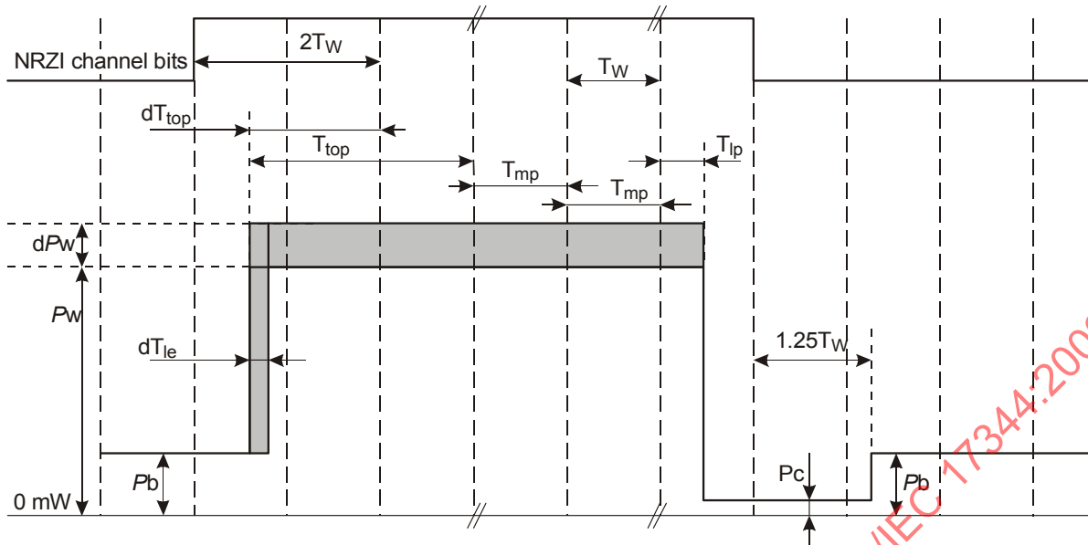
Figure G.3 — General blocked waveform
