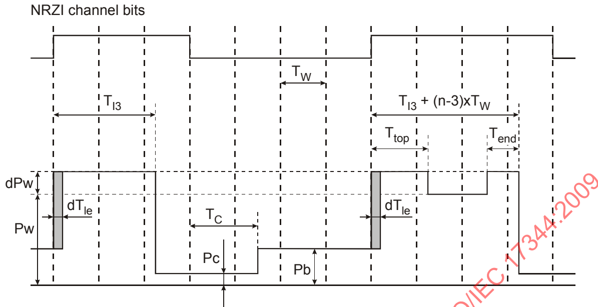
Figure G.5 — General Castle waveform
