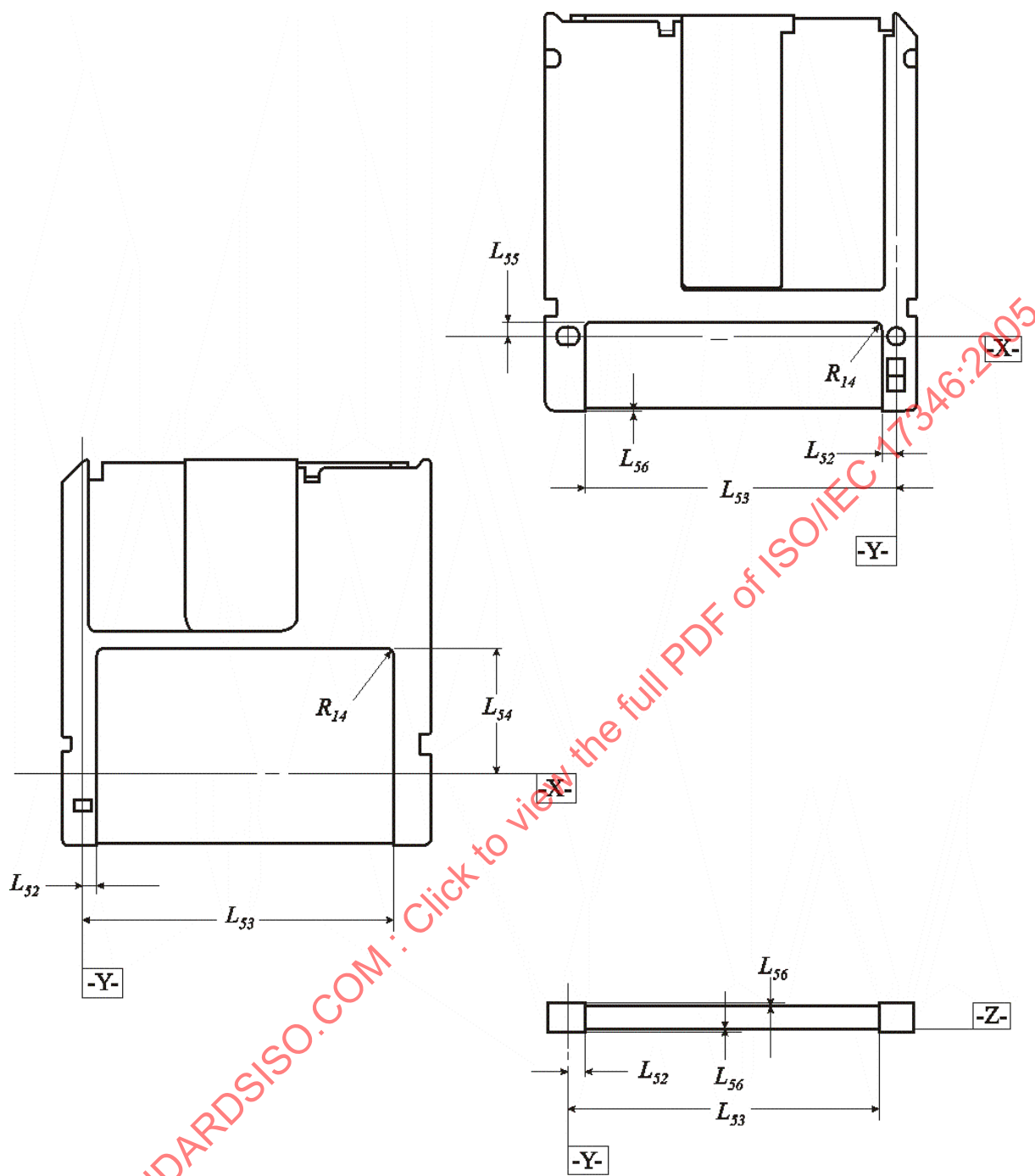
Figure 12 — Label area
