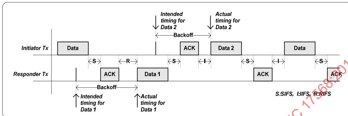
Figure 33 — Backoff procedure
