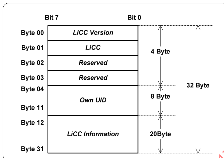
Figure 24 — Management Frame Body components
