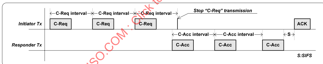
Figure 34 — C-Req transmission
