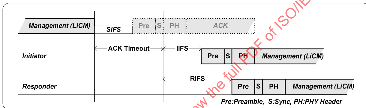
Figure 29 — Management frame (except C-Acc) ACK timeout &amp; retransmission
