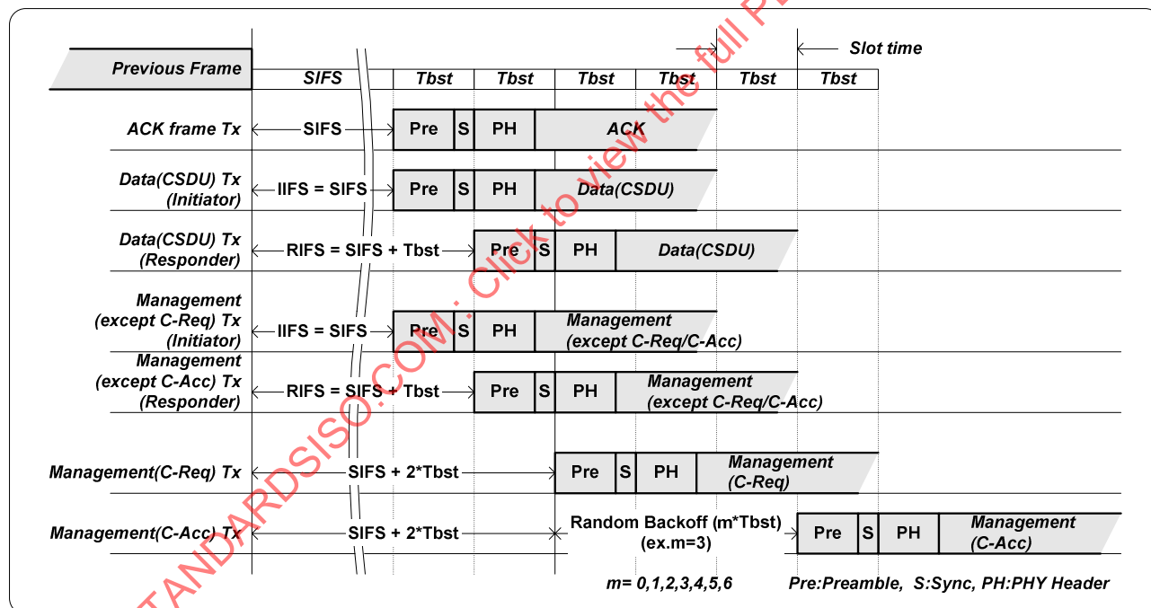
Figure 32 — Interframe space example
