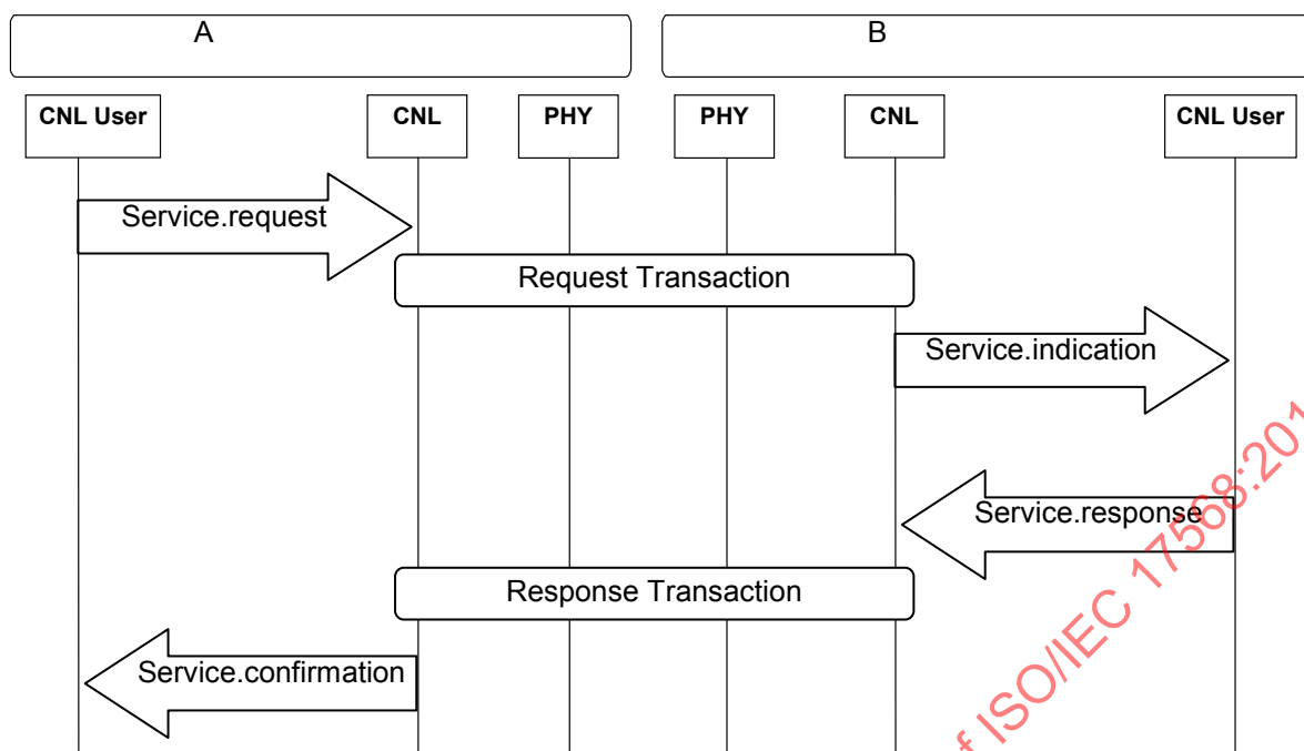
Figure 17 — CNL primitives between the CNL User and the CNL
