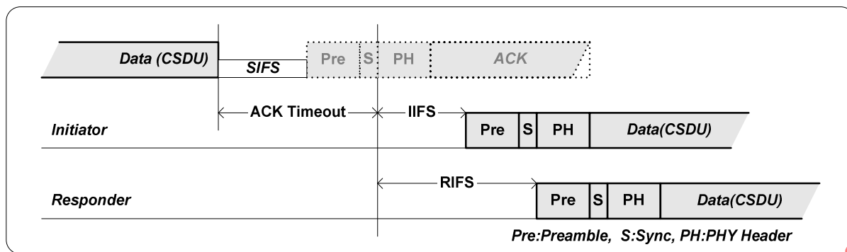
Figure 28 — Data frame ACK timeout &amp; retransmission
