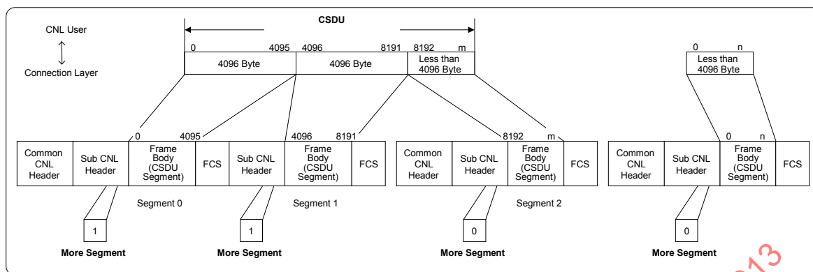
Figure 25 — Segmenting/Reassembling
