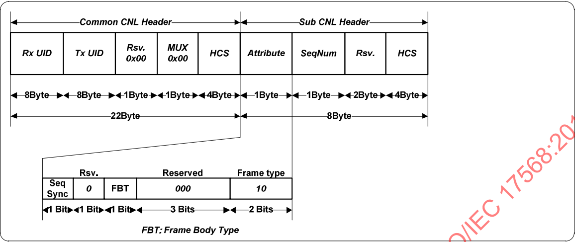
Figure 19 — ACK CPDU
