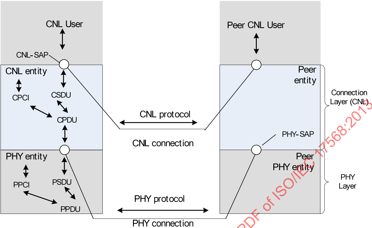
Figure 2 — OSI Basic Reference Model used in this International Standard
