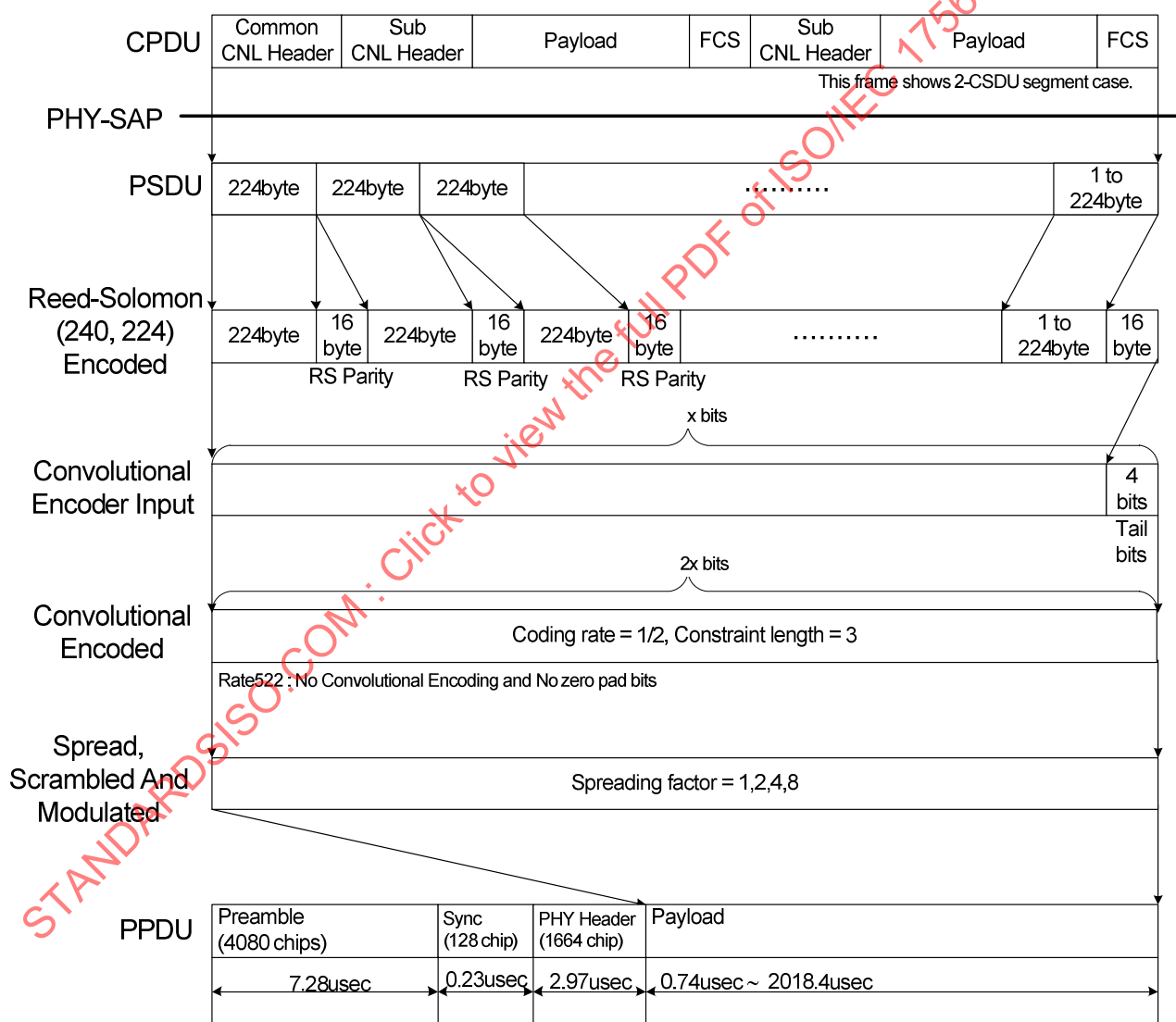
Figure 14 — CPDU encoding process and PPDU format
