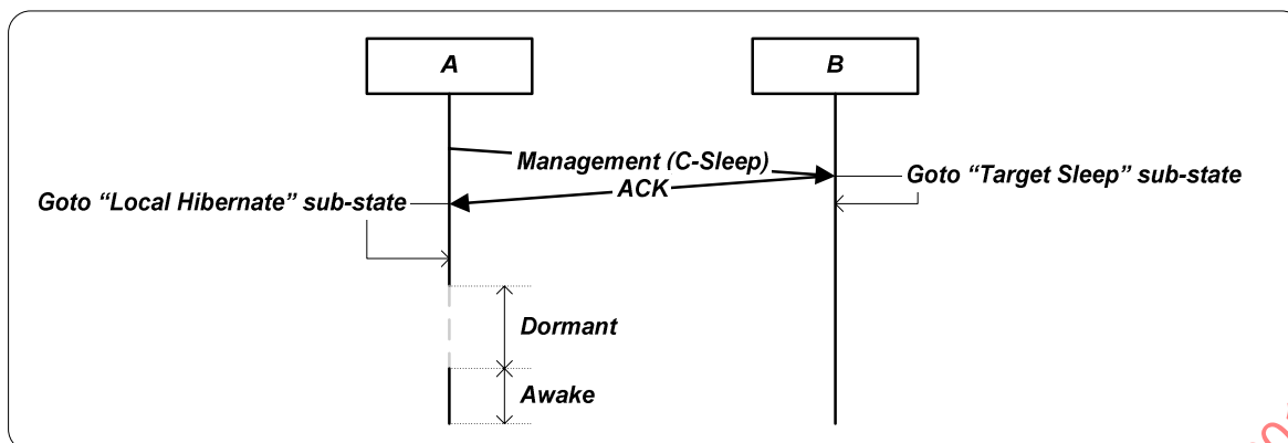
Figure F.4 — Connection sleep procedure (only the entity A performs the hibernation)
