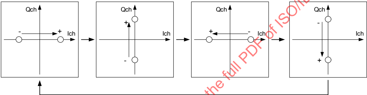
Figure 11 — Concept of Pi/2 shift BPSK
