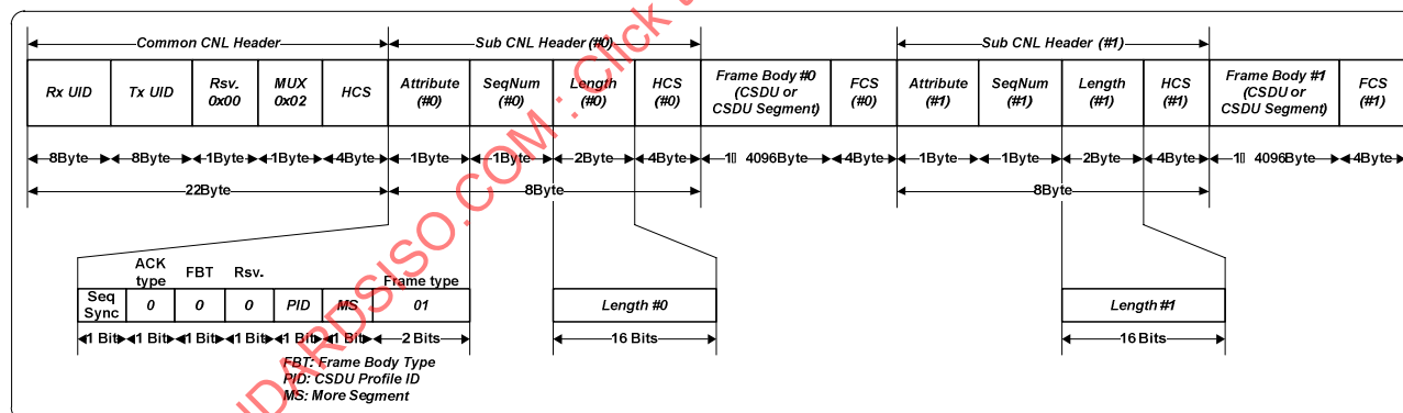
Figure 22 — Multi-Data CPDU
