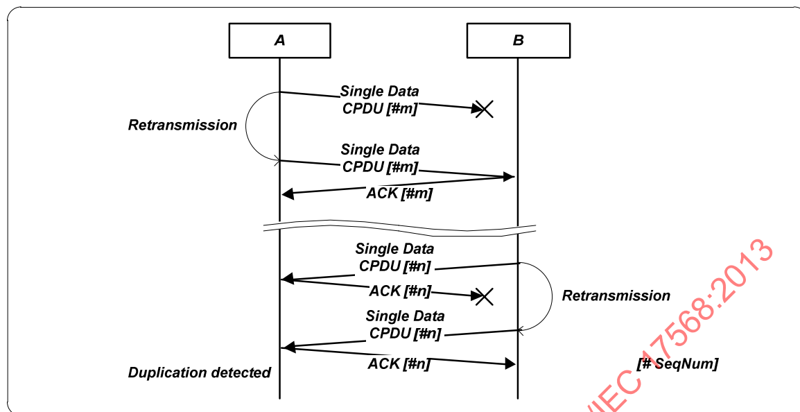
Figure F.2 — CSDU exchange procedure
