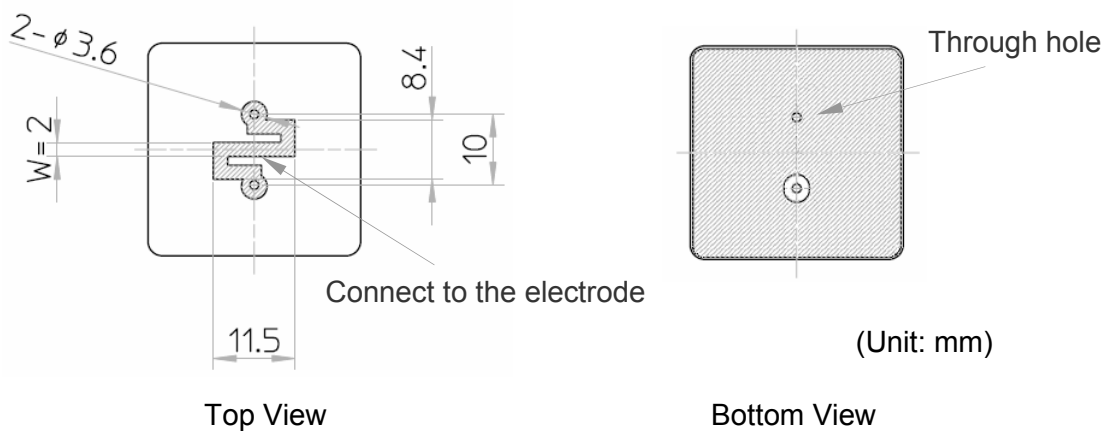
Figure D.2 — Printed wiring board pattern
