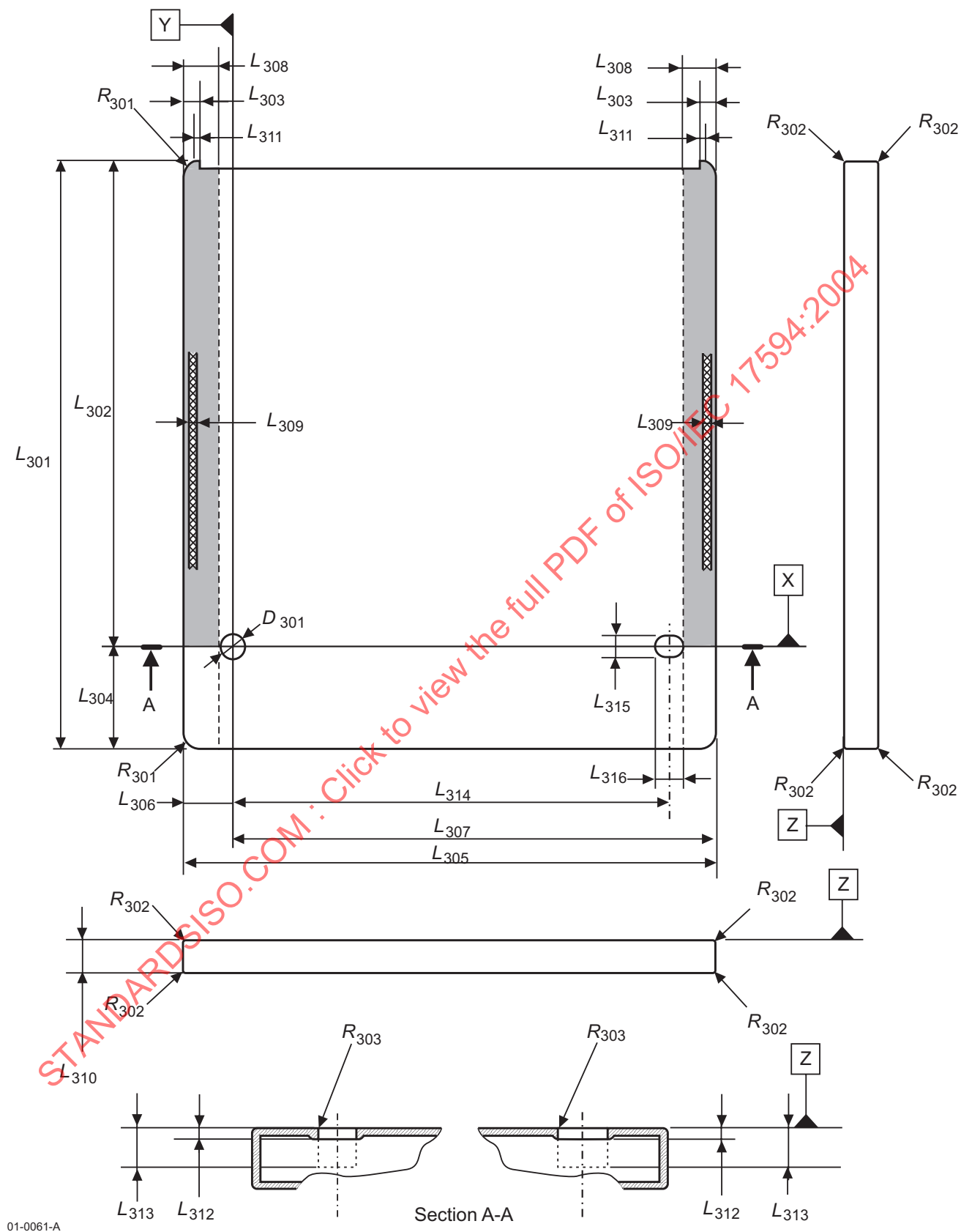
Figure 39 - Overall dimensions
