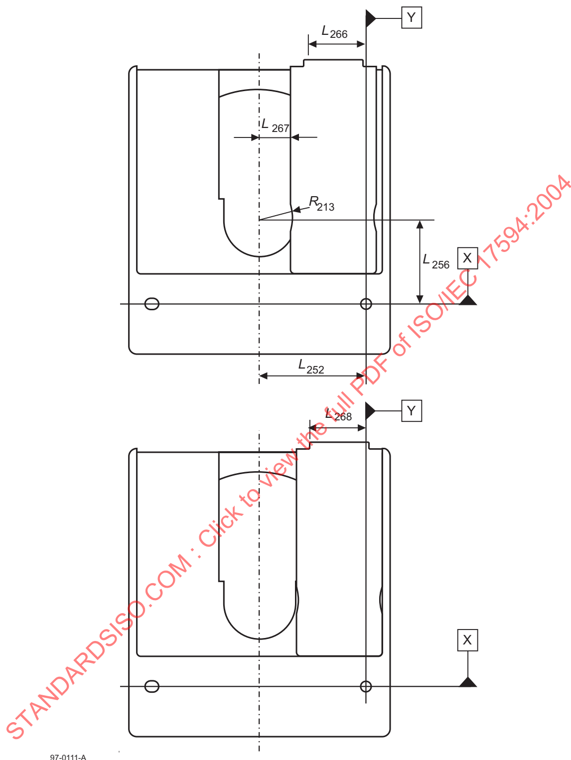
Figure 22 - Shutter in just right-hand open position (top view) and maximum right-hand open position (bottom view)
