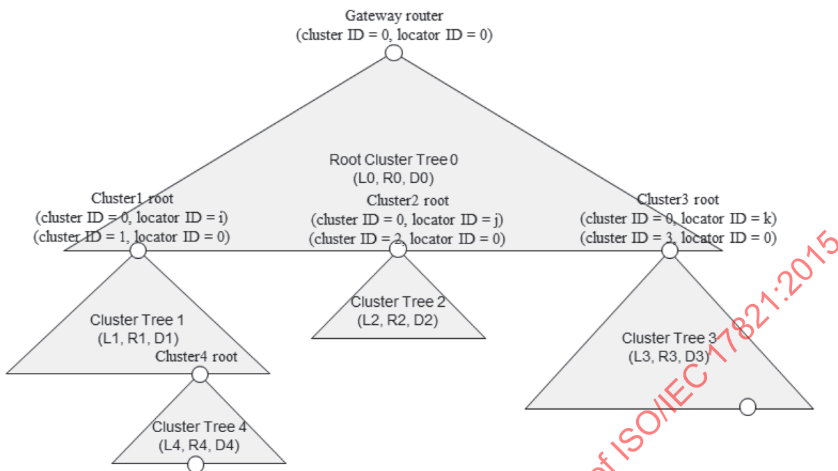
Figure 5.5 — Address assignment based on asymmetrical tree structure
