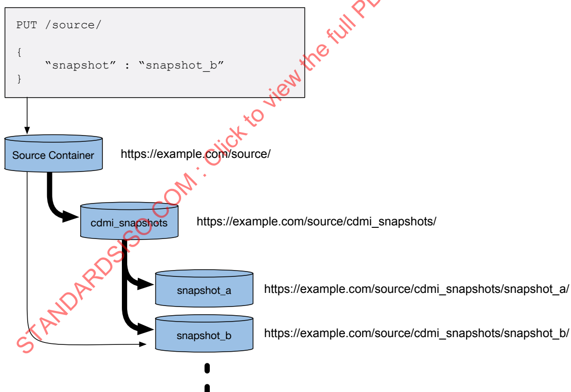
Fig. 10: Snapshot container structure
