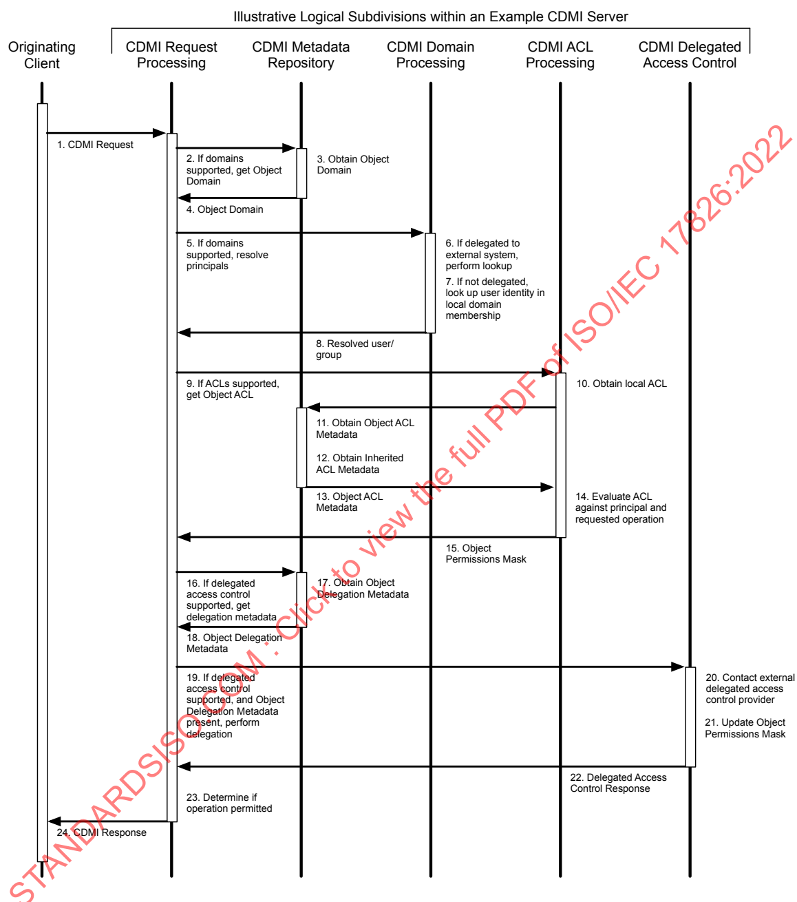
Fig. 11: Access control flow
