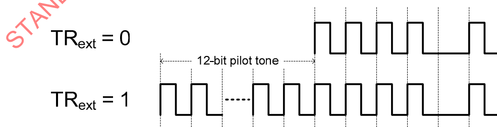
Figure 27 — ASK Method: FM0 Preamble SOF
