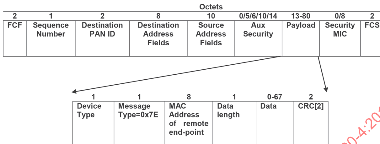
Figure 37 — Mesh data message format
