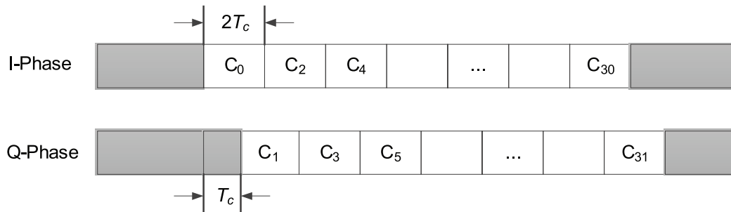
Figure 42 — O-QPSK modulation chips offset
