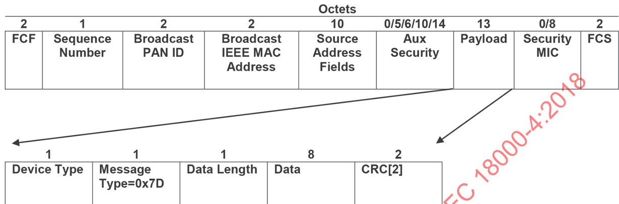
Figure 36 — Mesh request packet format
