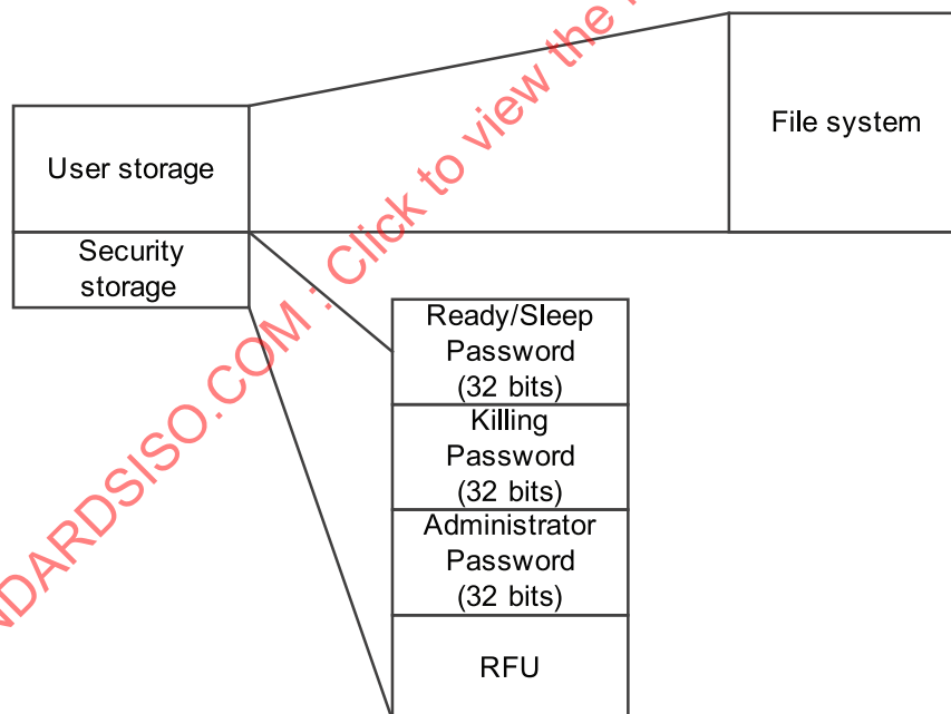
Figure 44 — Memory logic mapping
