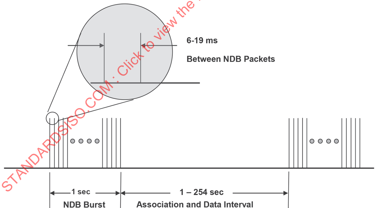
Figure 38 — NDB timing
