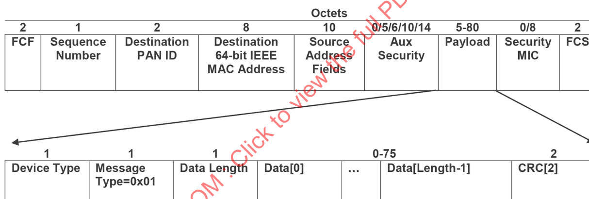
Figure 35 — Data message format
