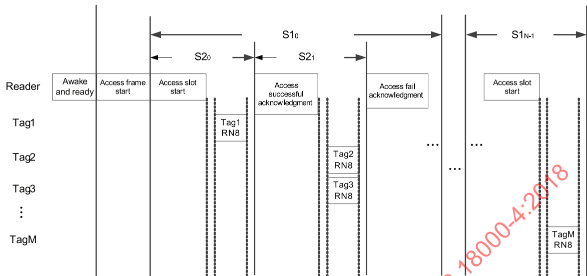
Figure 56 — Time-slot diagram in access stage
