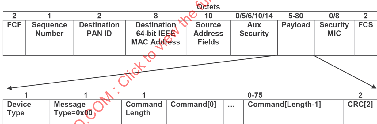
Figure 34 — Command packet format
