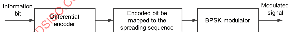
Figure 43 — DBPSK modulation and spreading functions
