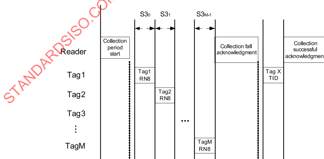
Figure 57 — Time-slot diagram in collection stage
