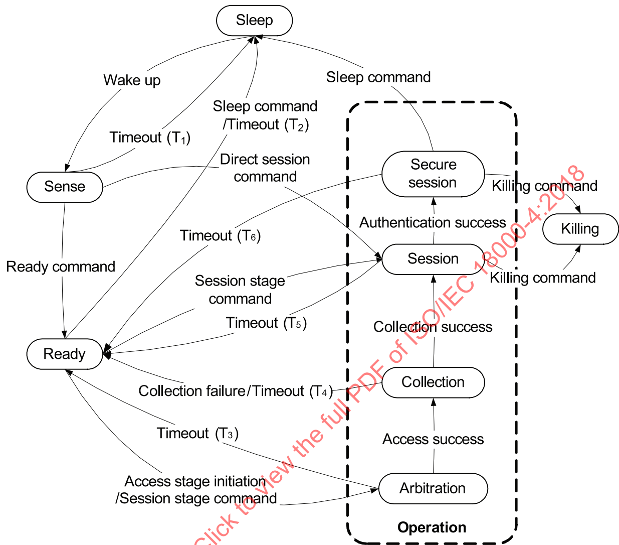
Figure 55 — Tag state transition
