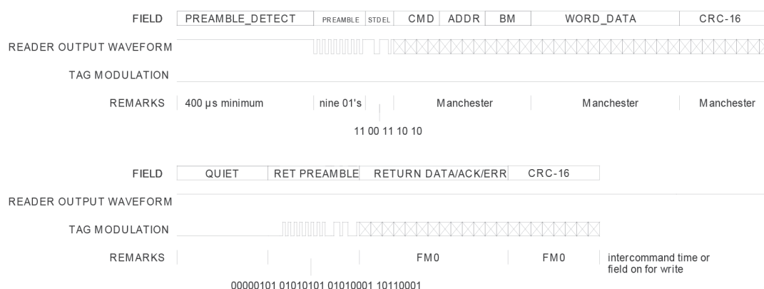
Figure 8 — Sample command/response packets for GROUP_SELECT (40 kbit/s on forward and return link)
