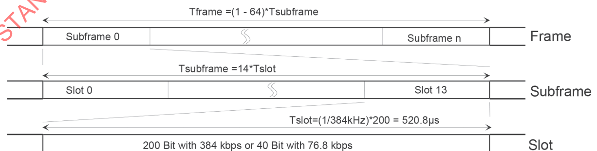
Figure 16 — Frame structure
