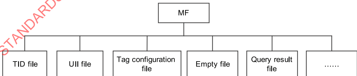
Figure 48 — File directory structure
