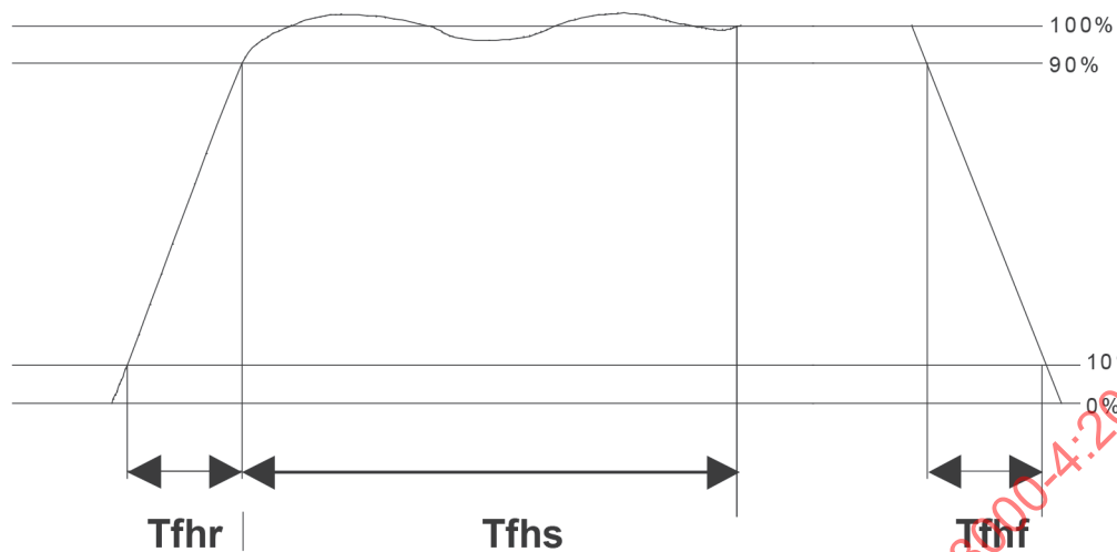
Figure 3 — FHSS carrier rise and fall characteristics
