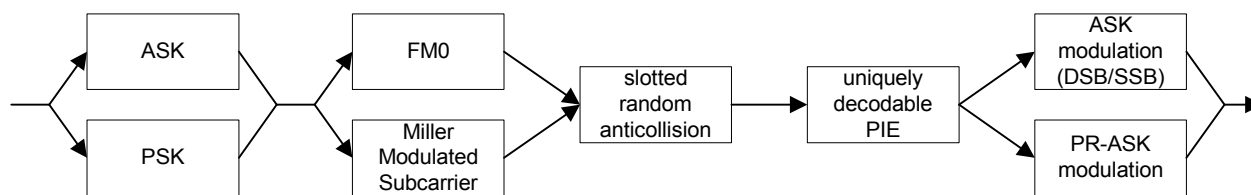
Figure 3 — Type C Interrogator architecture
