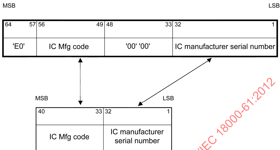
Figure 12 — Tag ID/SUID mapping from 64 to 40
