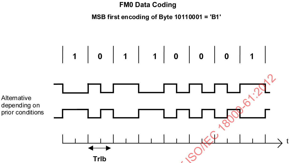
Figure 4 — Tag to Interrogator data coding
