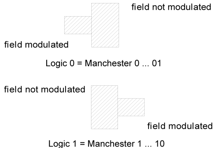
Figure 9 — Forward link bit coding
