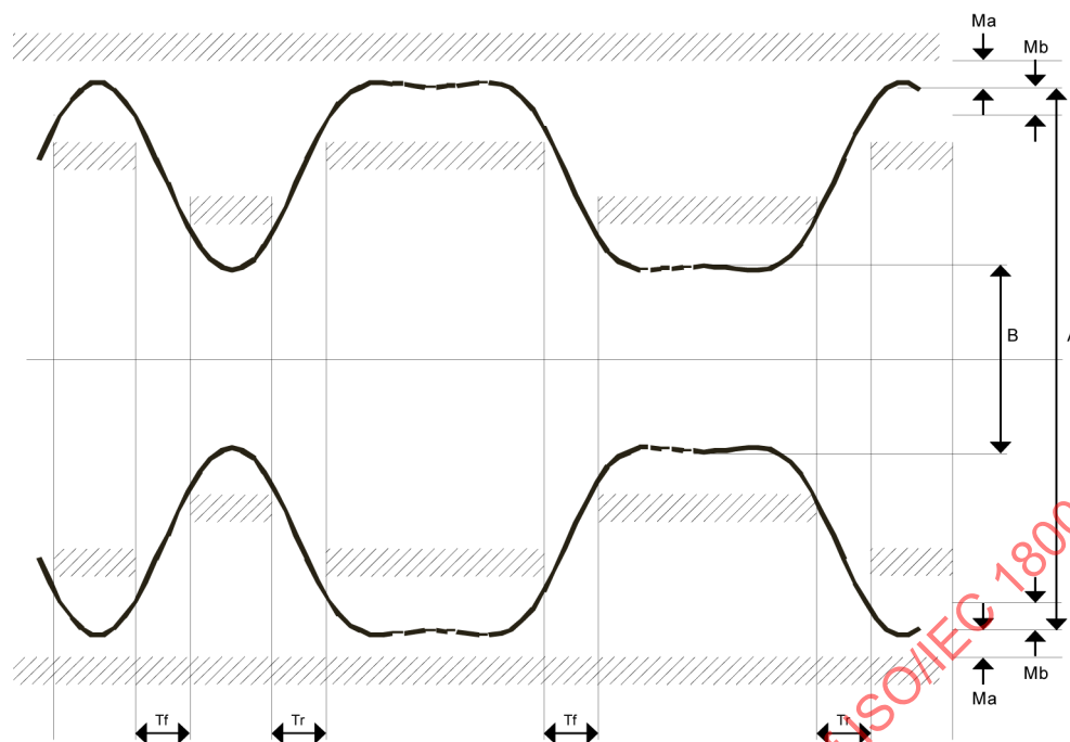
Figure 8 — 18% modulation (example of 8 kbit/s signal)
