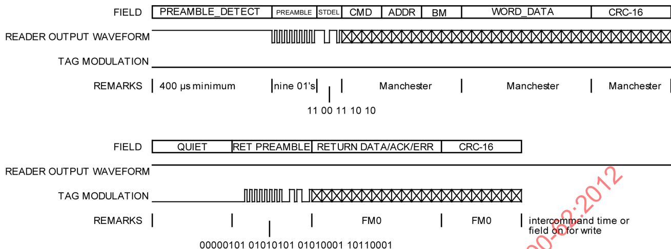
Figure 12 — Sample command/response packets for GROUP_SELECT (40 kbit/s on forward and return link)
