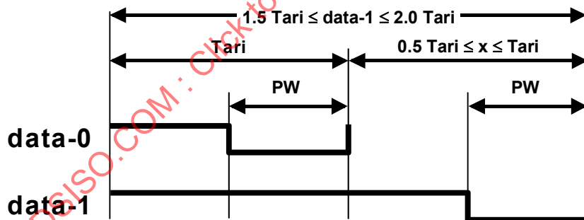
Figure 1 — PIE Symbols
