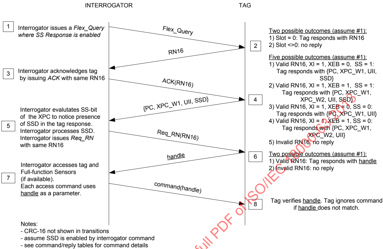
Figure E.4 — Example of Tag inventory and access if Simple Sensor Data Block is provided
