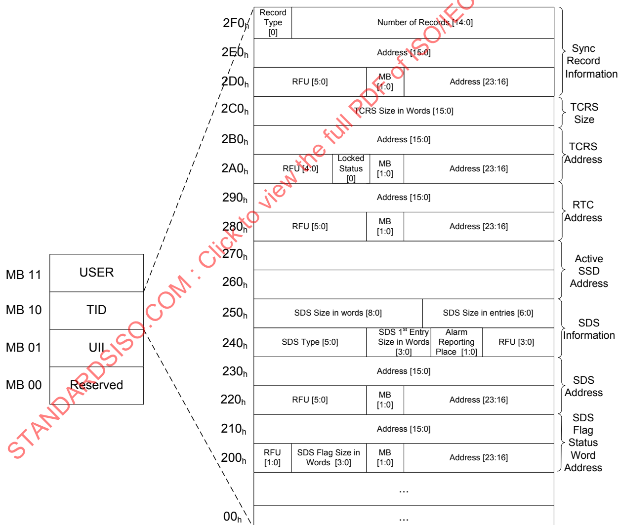
Figure 39 — Structure of TID memory
