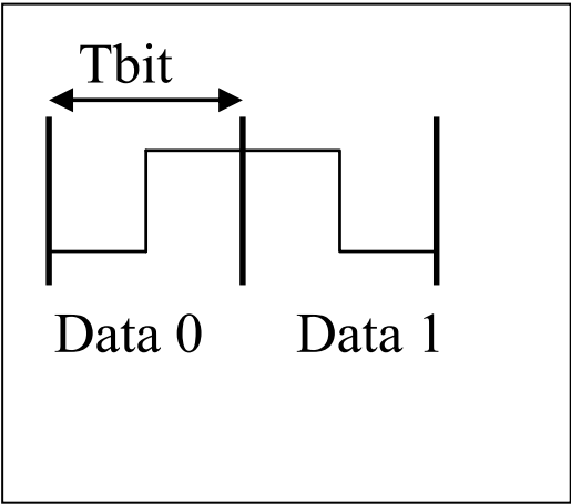
Figure 27 — Manchester symbols
