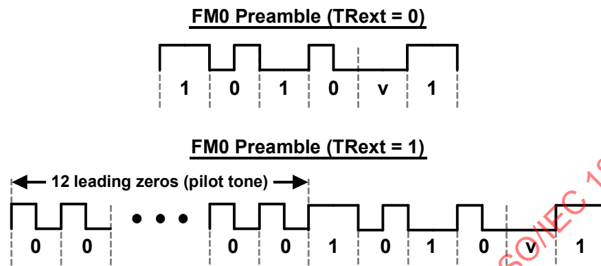
Figure 11 — FM0 T=&gt;R preamble
