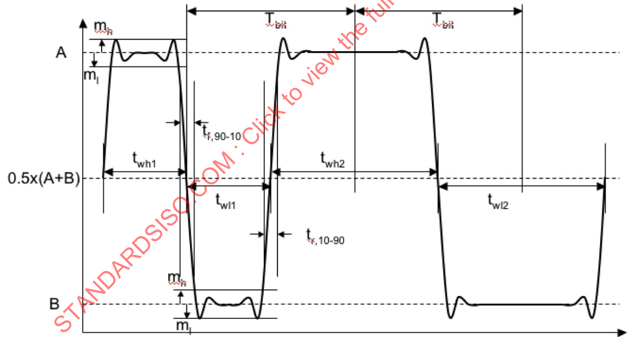
Figure 28 — Manchester waveform
