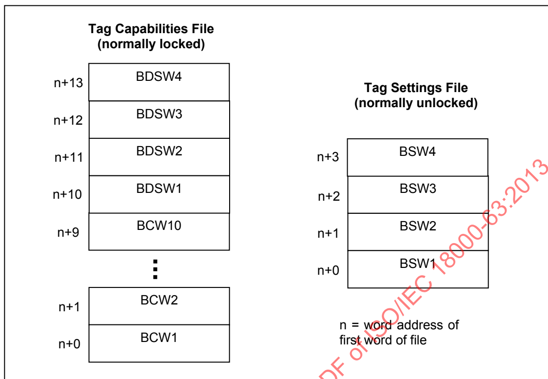
Figure 38 — Structure of Tag Capabilities and Tag Settings Files for Version Code = 1.
