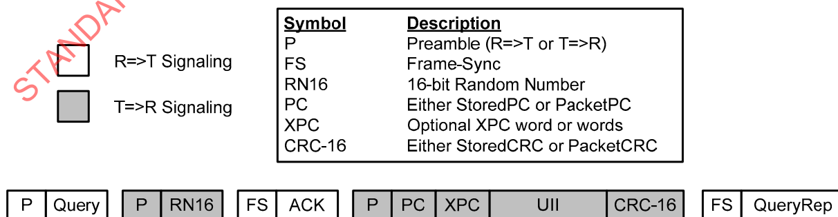
Figure 21 — One Tag reply
