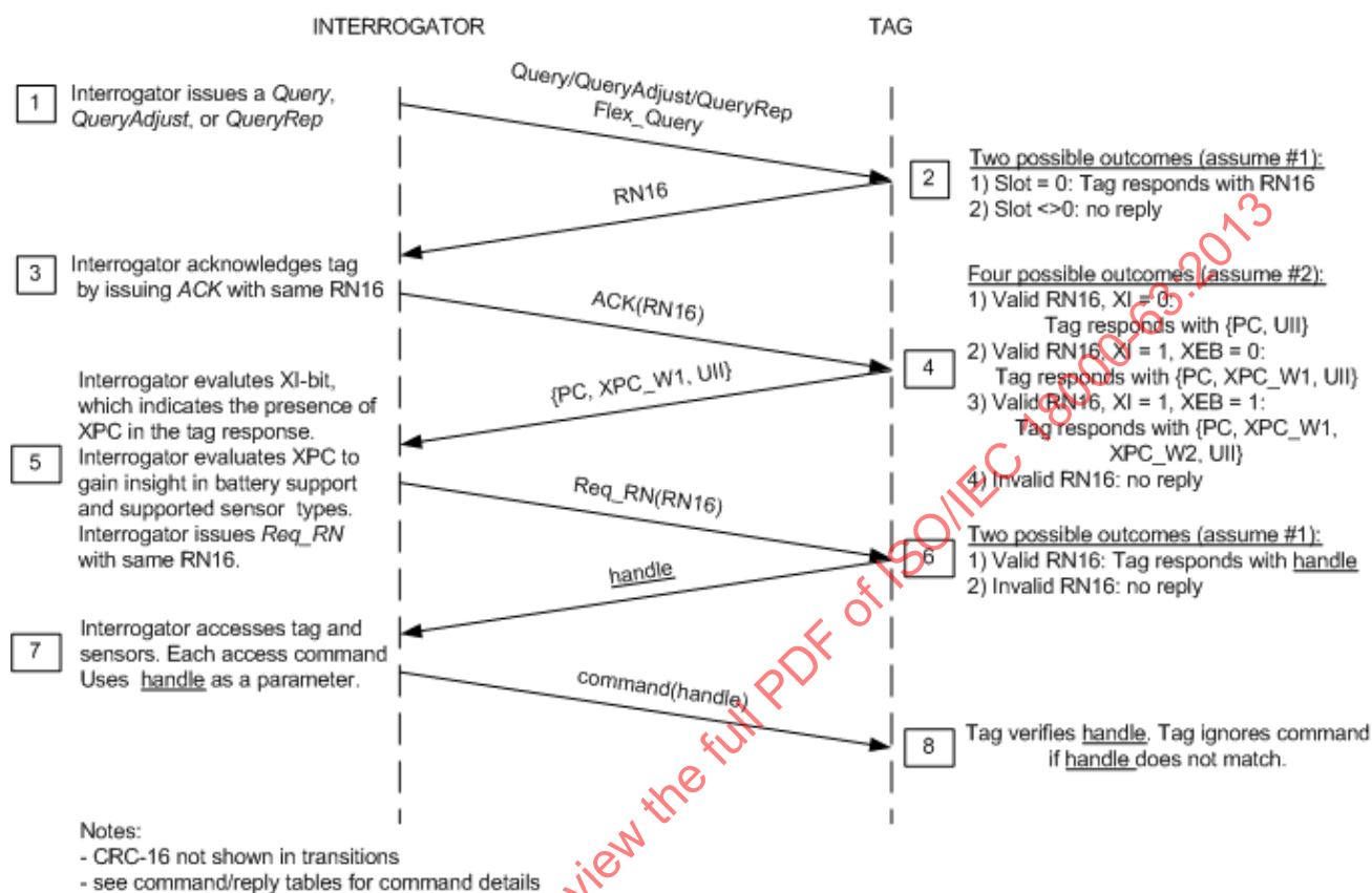
Figure E.2 — Example of Tag inventory and access if bit 16 h (XI) in the UII memory is asserted
