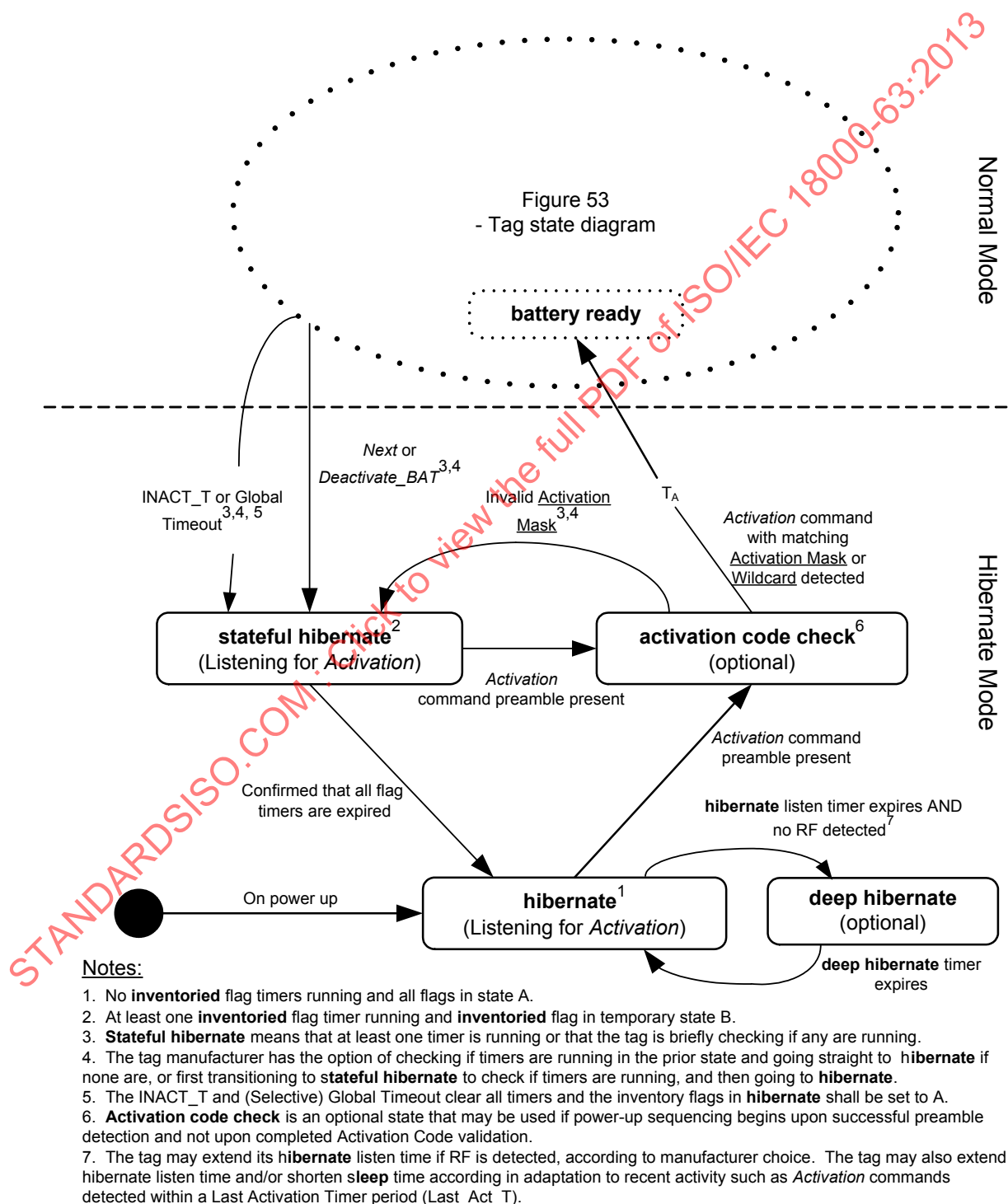
Figure 34 — Extended state machine of BAP Tag implementing Manchester mode
