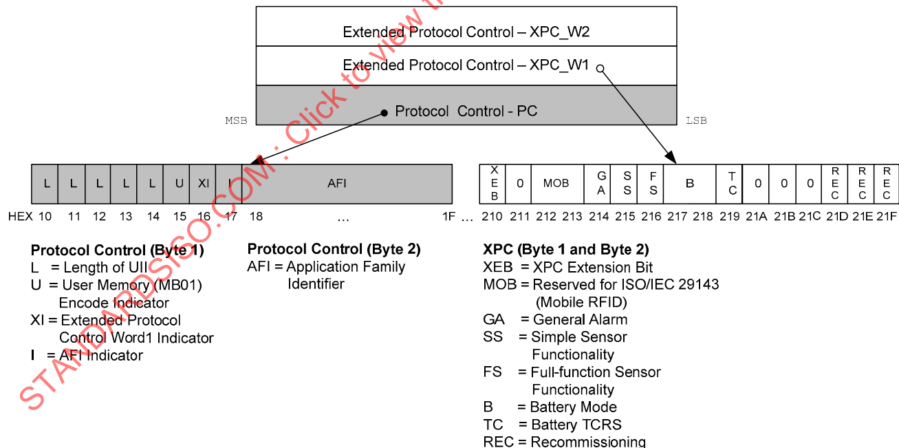
Figure 36 — Extended Protocol Control bit definitions (see NOTES 1 and 2)
