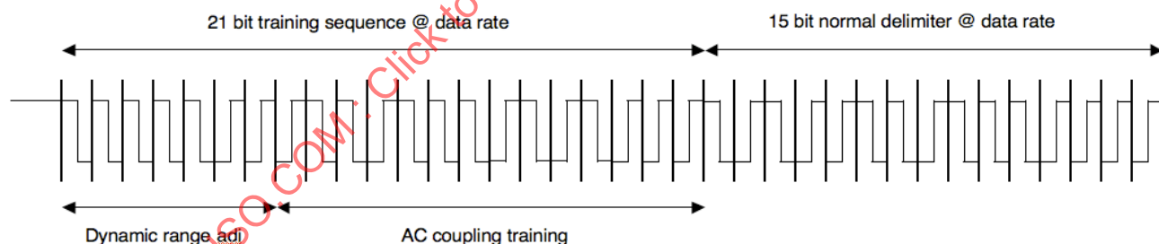
Figure 29 — Forward (R=>T) preamble
