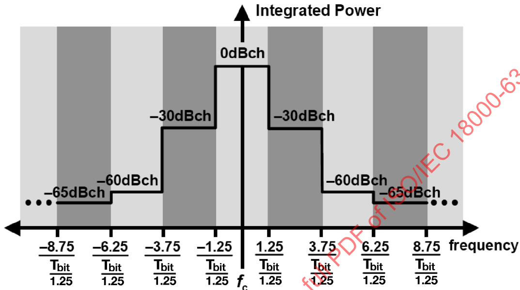
Figure 30 — Transmit mask for Manchester battery assisted mode
