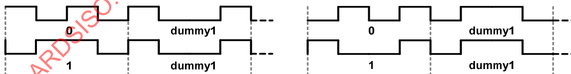
Figure 10 — Terminating Miller (M=2) subcarrier transmissions
