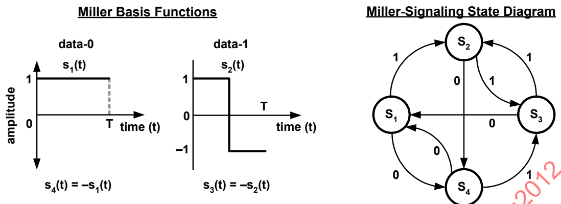
Figure 8 — Miller basis functions and generator state diagram
