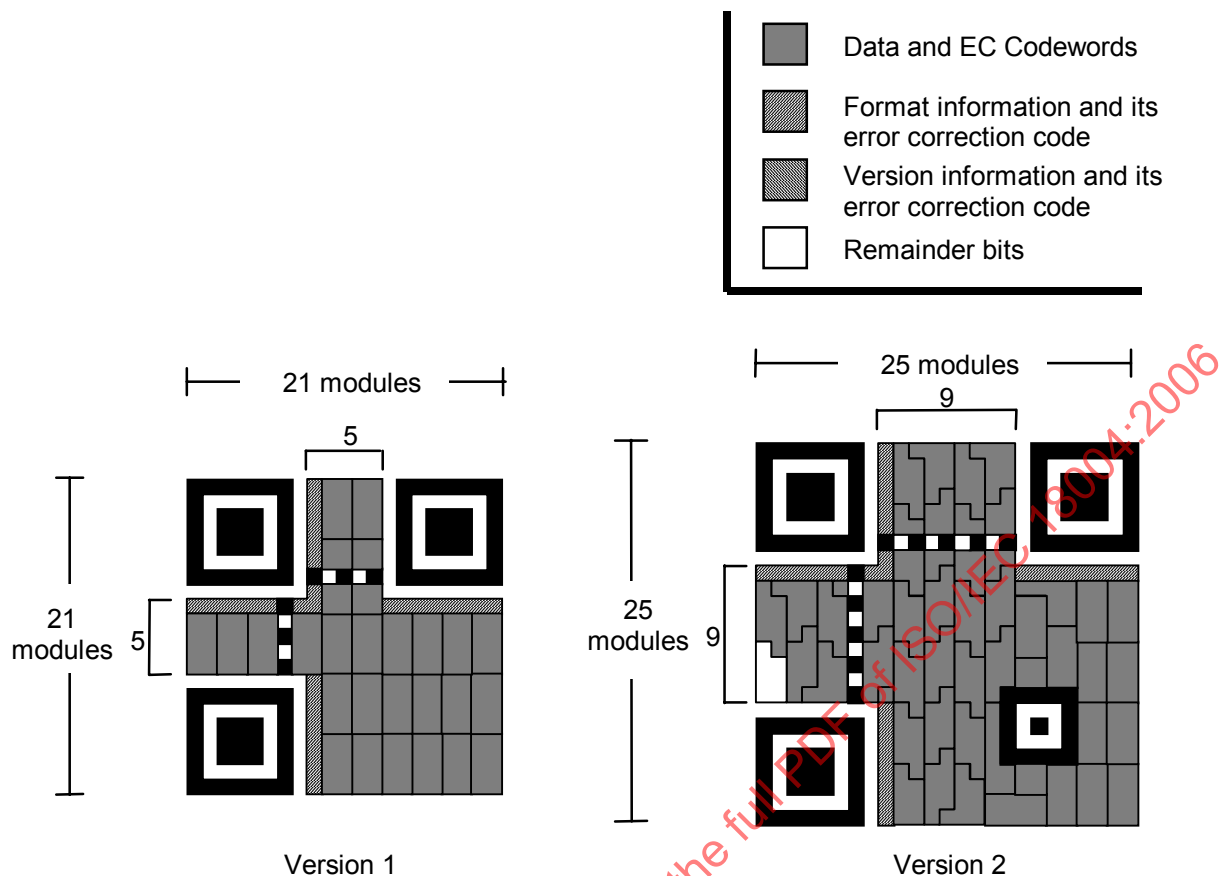
Figure 5 — Version 1 and 2 symbols
