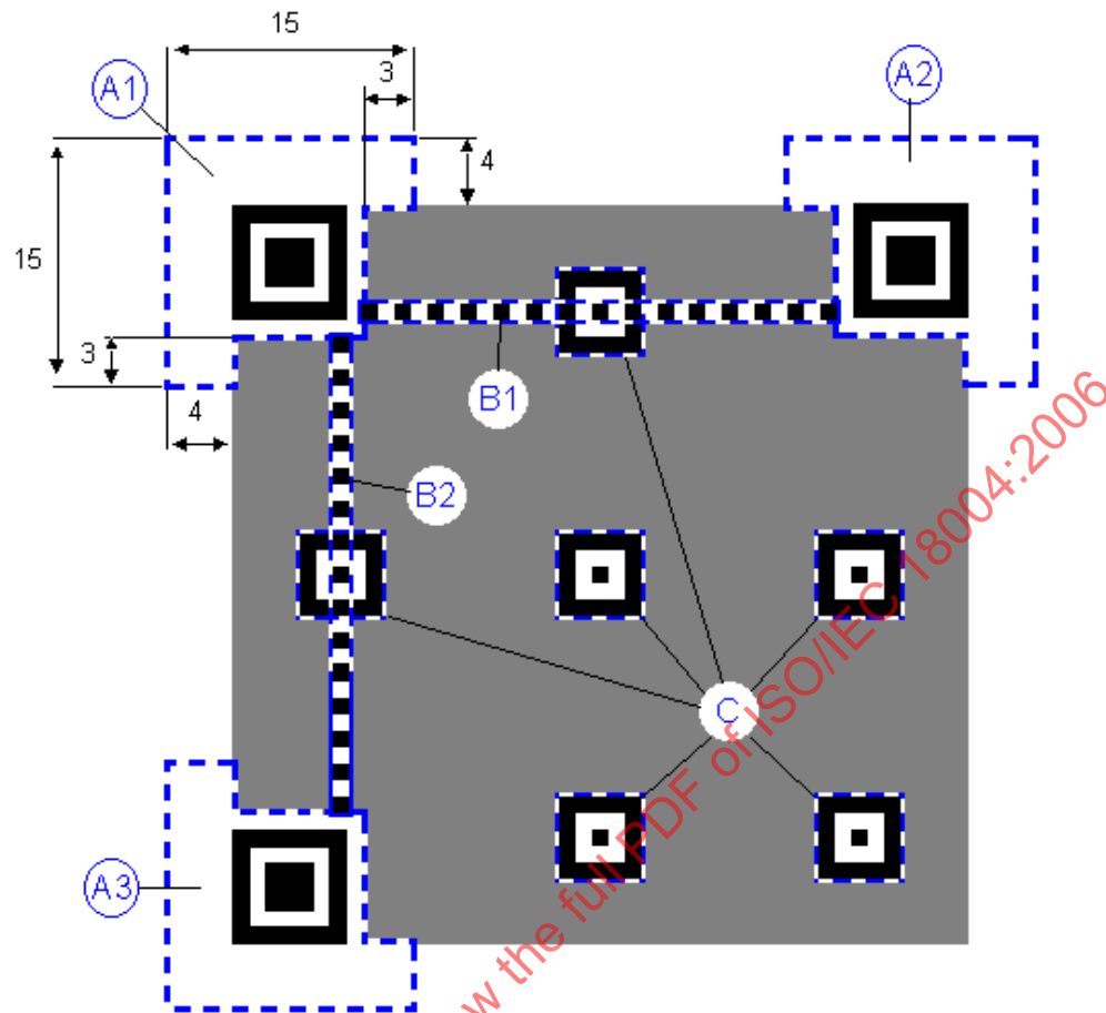
Figure G.1 — QR Code 2005 fixed pattern segments
