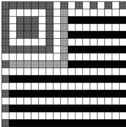
a) Mask pattern 00
