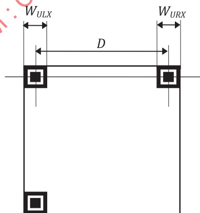
Figure 32 — Upper finder patterns
