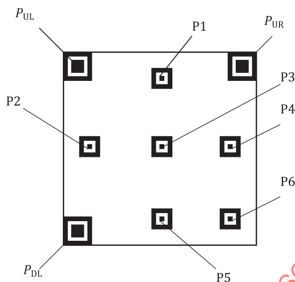
Figure 34 — Finder patterns and alignment patterns
