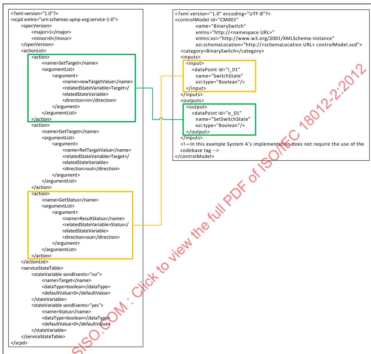
Figure A.9 – Functional mapping of SwitchPower service to the LightLamp
