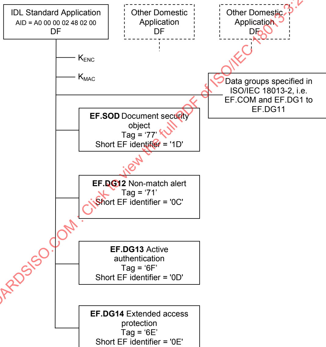
Figure 15 — Data groups
