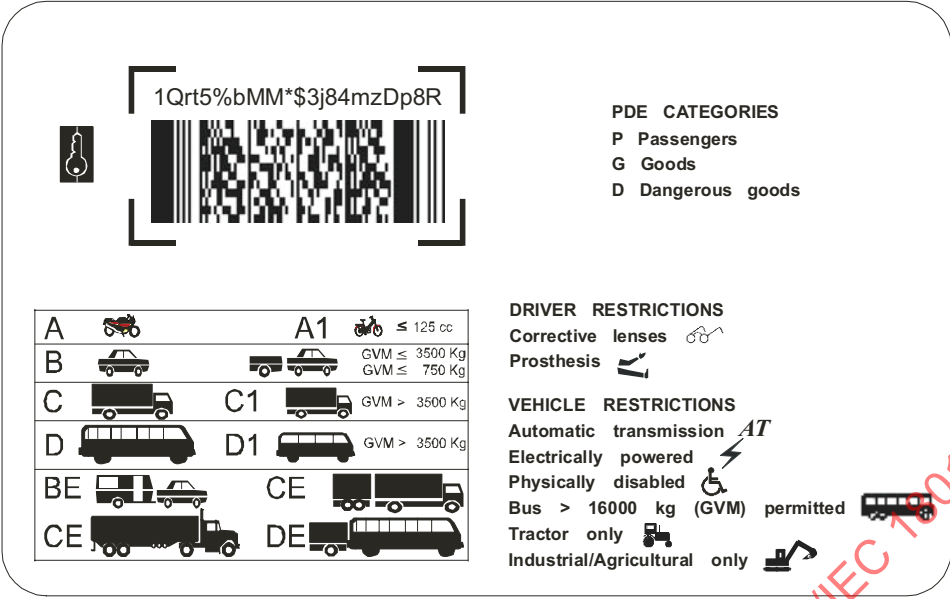
Figure 17 — Basic access protection logo on IDL (not to scale)
