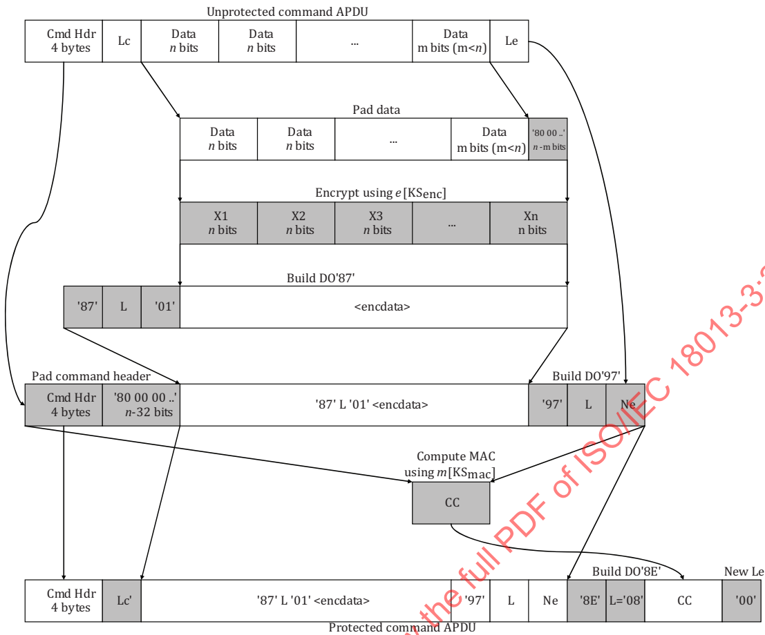
Figure B.1 — Computation of a SM command APDU
