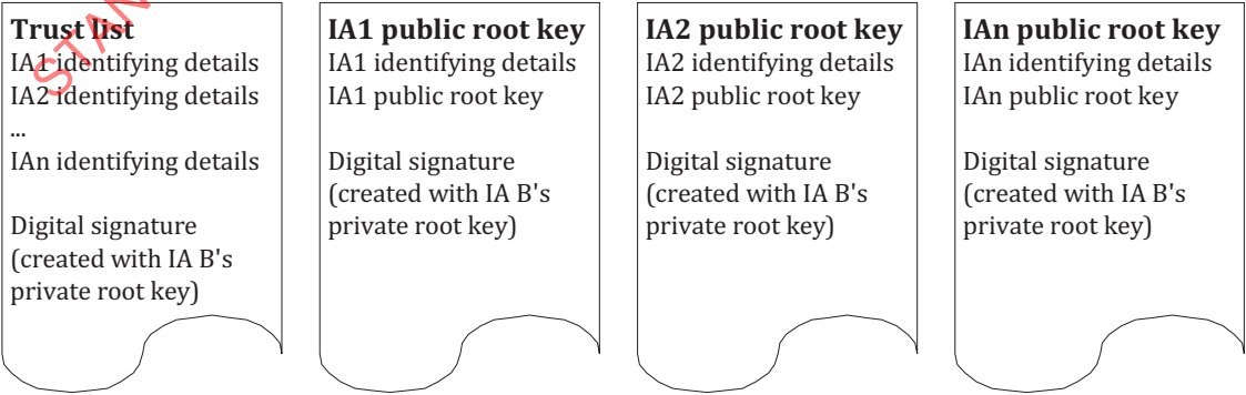
Figure A.1 — Certificates published by an IA
