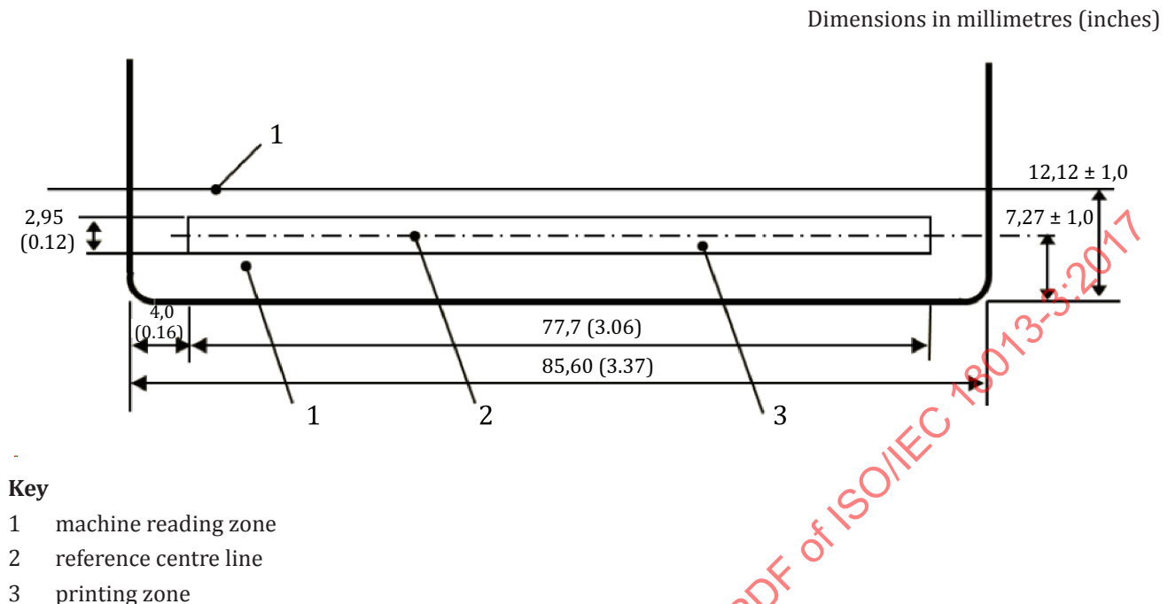
Figure 13 — Location of 1 line MRZ at the bottom of the IDL (not to scale)
