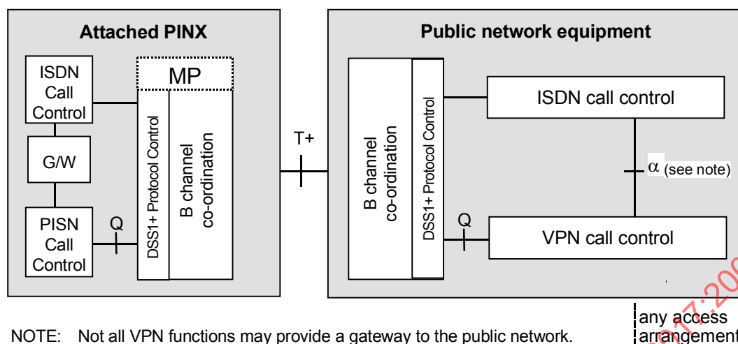
Figure 4 - Shared access arrangement using an enhance ISDN access protocol (DSS1+)
