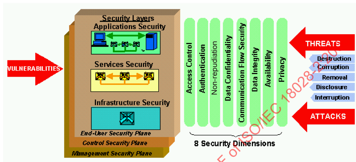
Figure 3 — Reference Architecture for End-to-End Network Security
