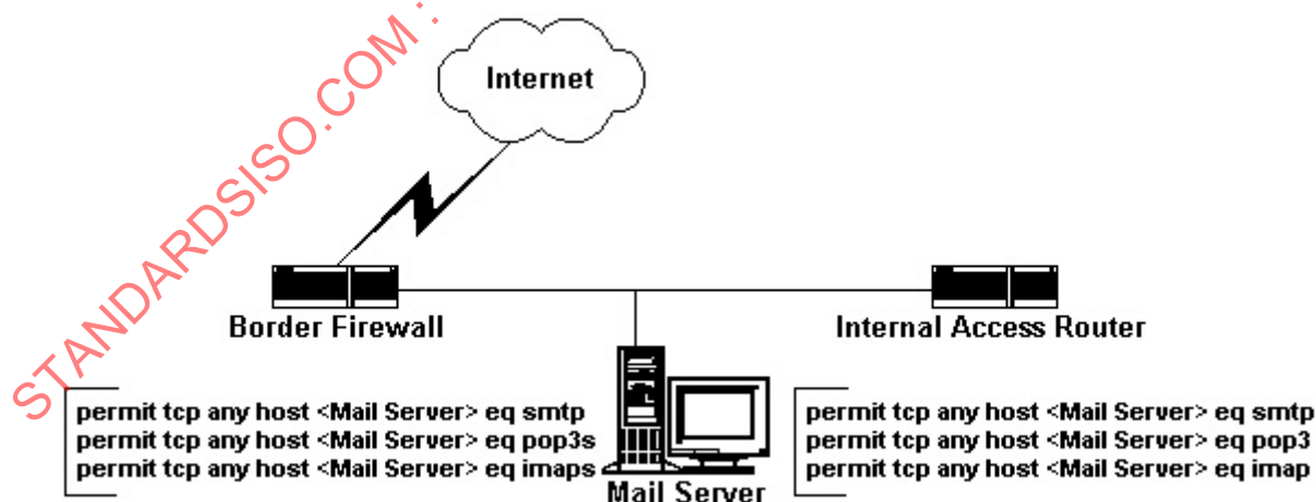
Figure 3 — Access to a Mail Server within a DMZ
