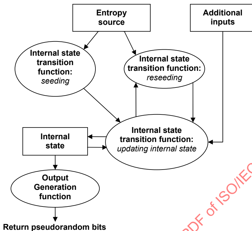
Figure 5 — DRBG model
