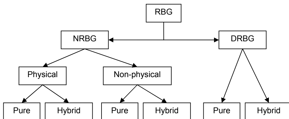
Figure 2 — RBG classes
