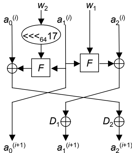
Figure 6 — \rho function of MUGI
