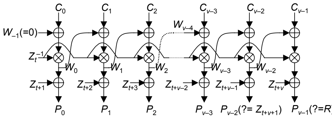
Figure 2 — Out^{-1} function of MULTI-S01 mode
