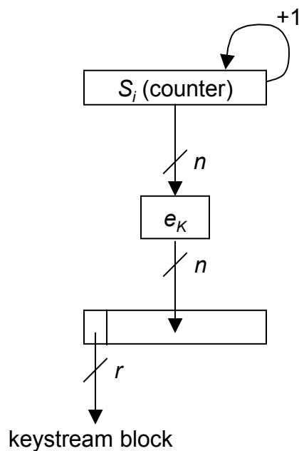
Figure 4 — Keystream generation based on CTR mode
