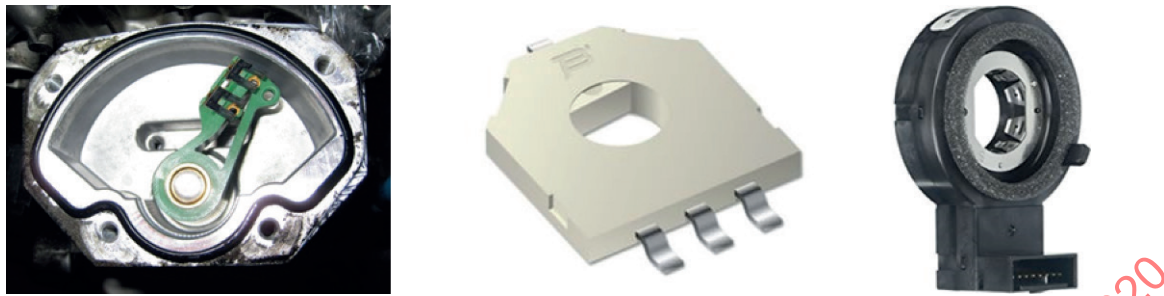
Figure 13 — Position sensors
