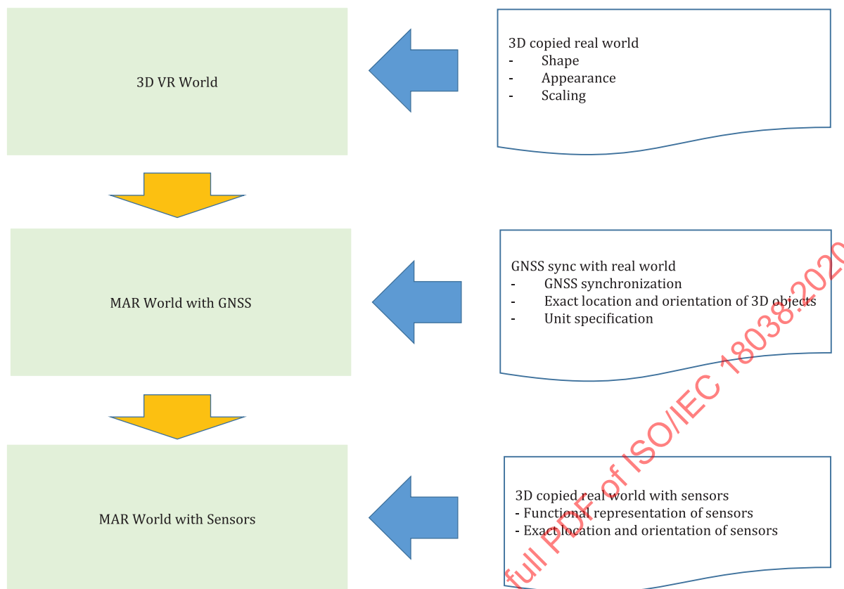
Figure 19 — Creation of a sensor MAR world
