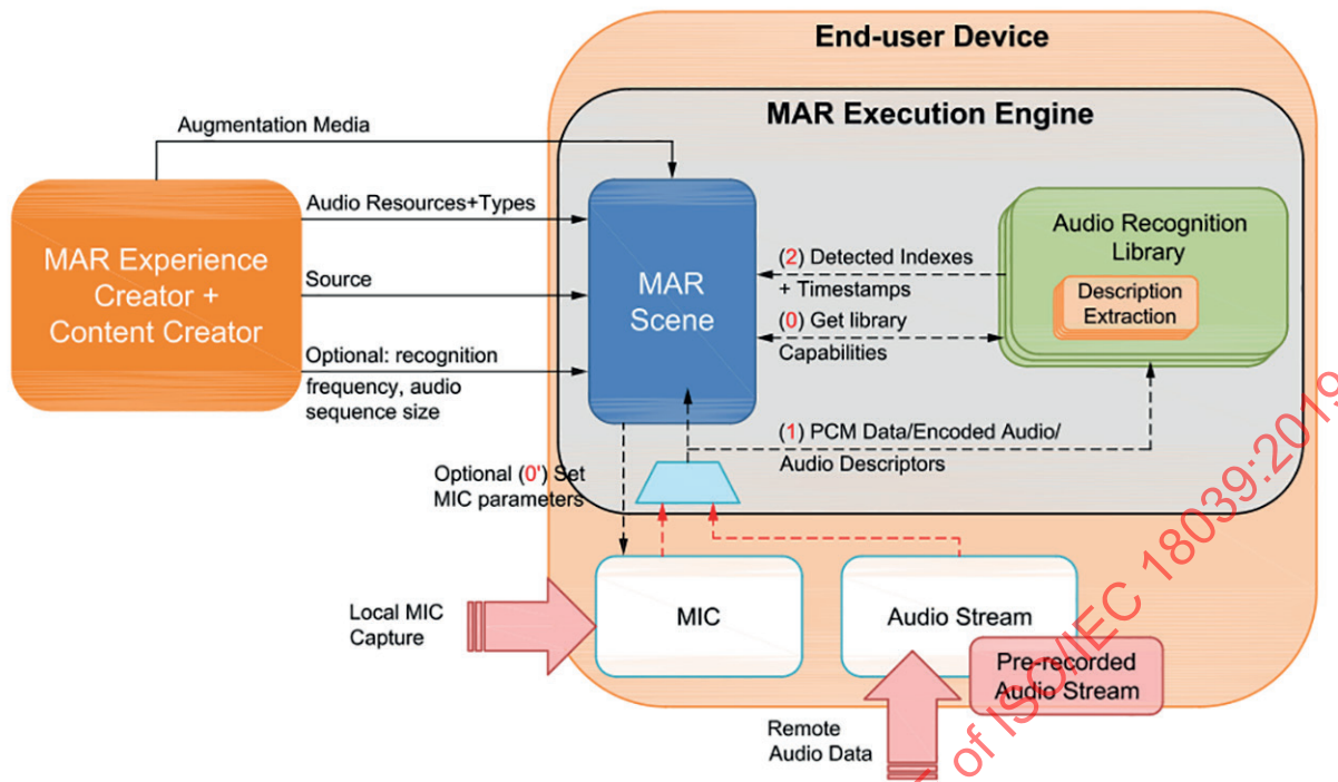
Figure 18 — Remote audio recognition
