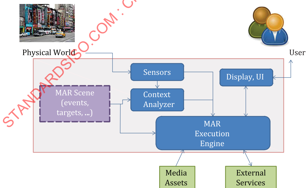
Figure 4 — Major components and their interconnection in an MAR system at a high macro level
