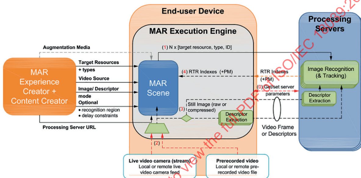
Figure 8 — Local registration, remote recognition and tracking
