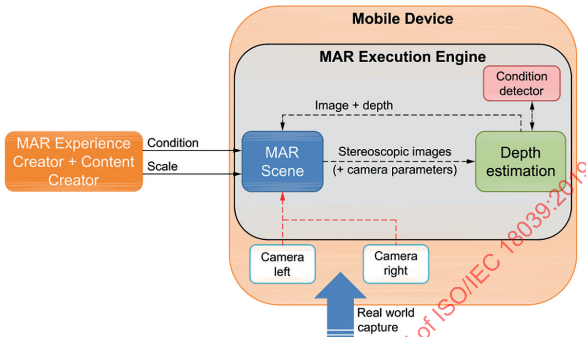
Figure 11 — Real-time, local depth estimation, condition based augmentation
