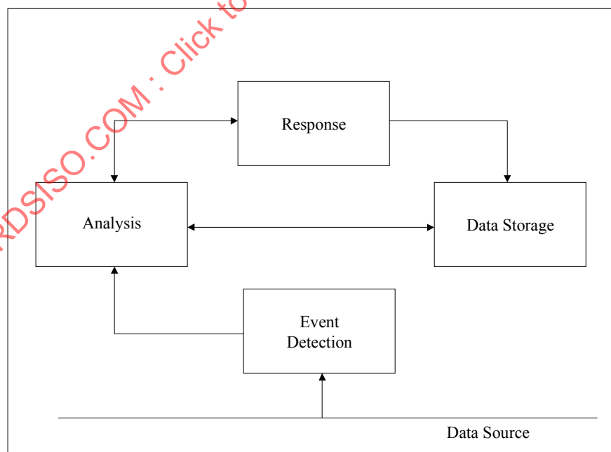
Figure A.1 — Generic model of intrusion detection
