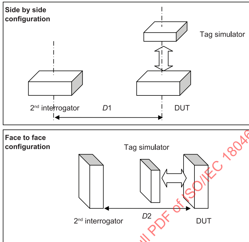
Figure 2 — Test configurations
