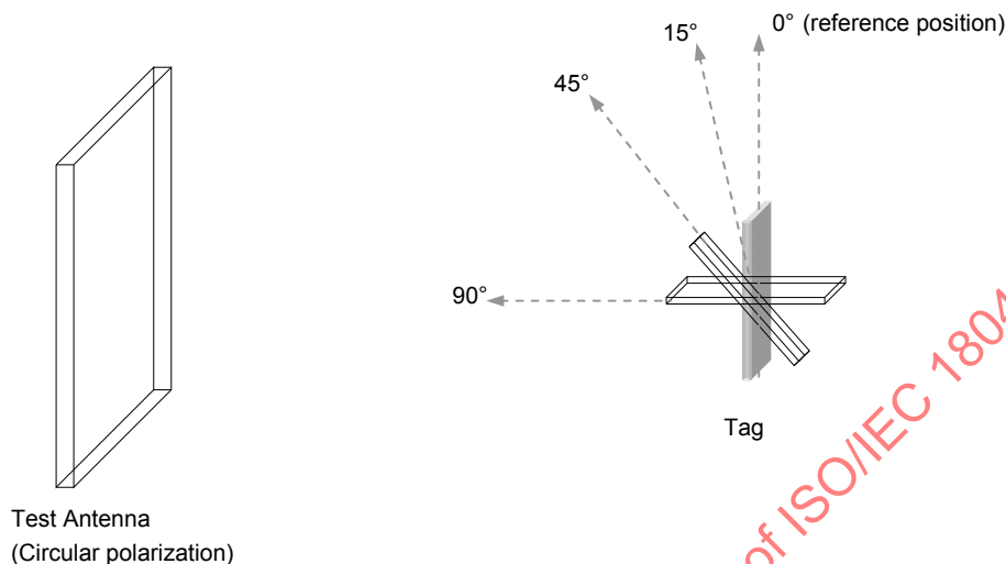
Figure 3 — Elevation tag orientations (Front view)
