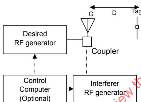
Figure 2 — Test set-up for interference rejection measurement
