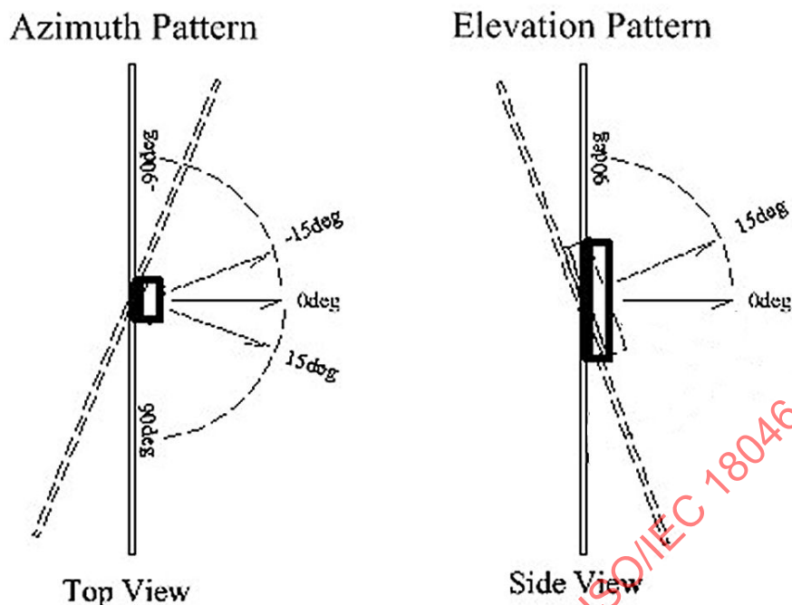
Figure 6 — Azimuth and elevation pattern
