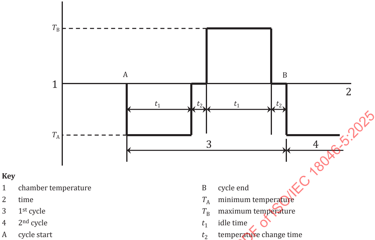
Figure 2 — Temperature change test cycle configuration
