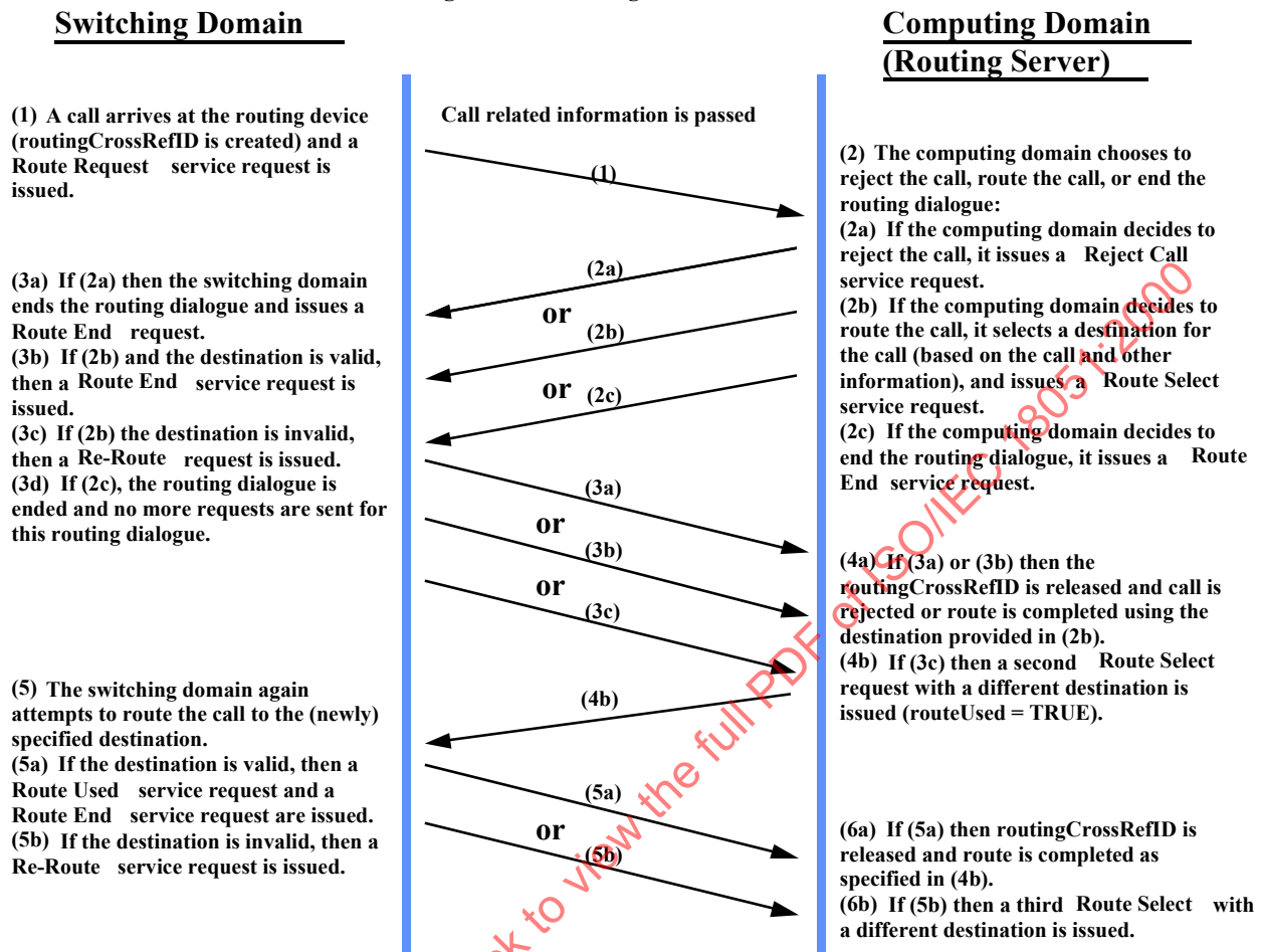
Figure 6-28 Routeing Procedure
