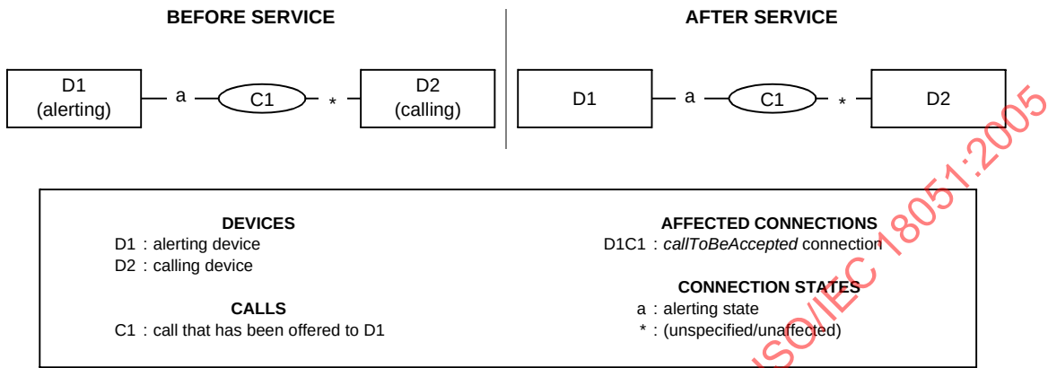
Figure 17-1 Accept Call Service
