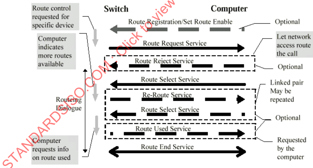
Figure 6-31 Overview of a Routing Dialogue
