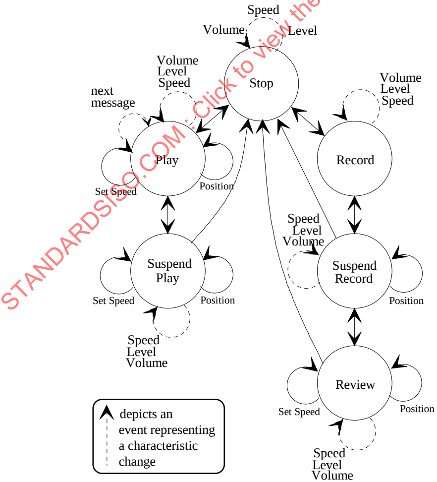
Figure 6-16 Voice Unit Operational Model
