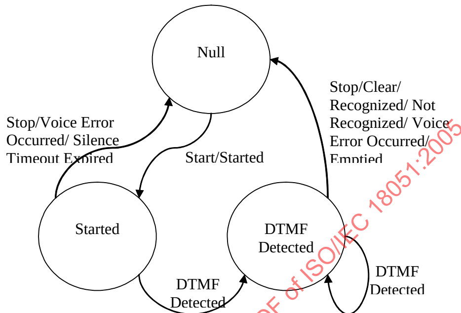
Figure 6-18 DTMF Resource Operational Model
